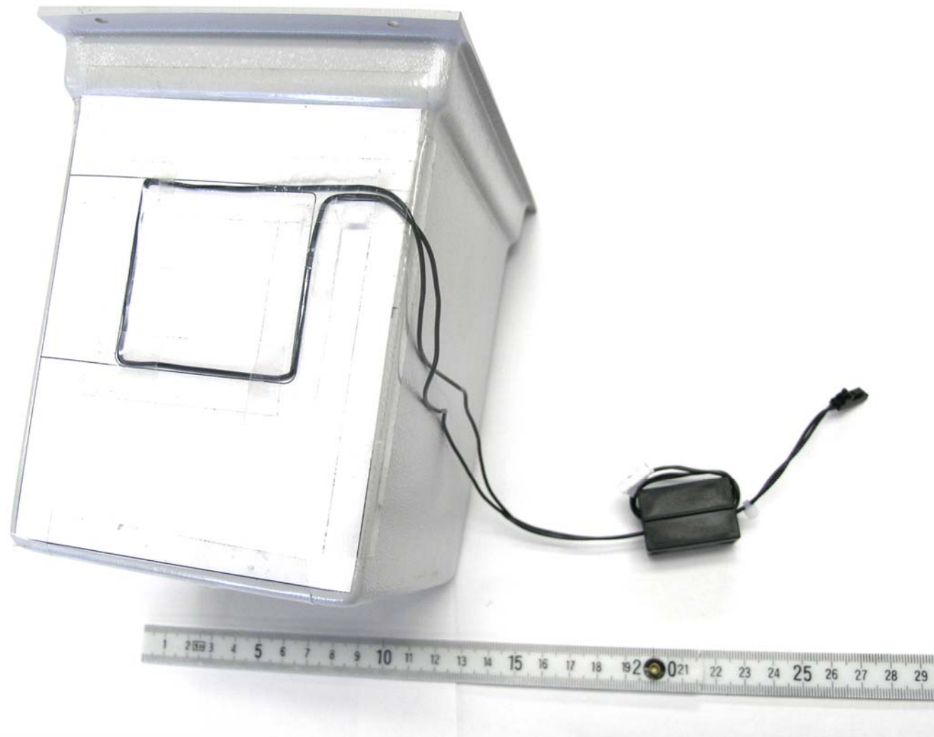
Custom Loop Antenna
