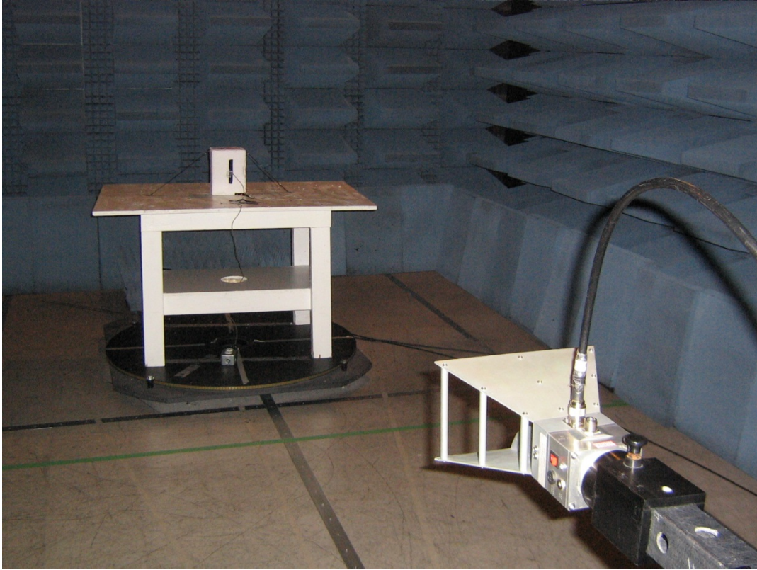
Radiated Emission Test Setup in the Semi-Anechoic Chamber: NCZ-3014/3031
