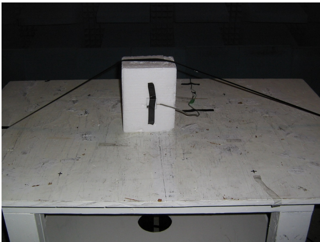
Radiated Emissions Test Set-Up in the Semi-Anechoic Chamber: NCZ-3014/3031
