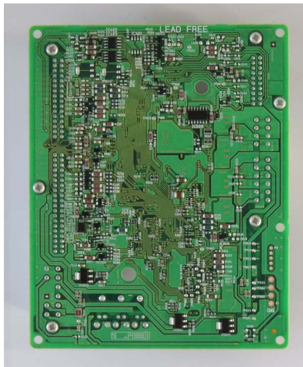
Solder side
