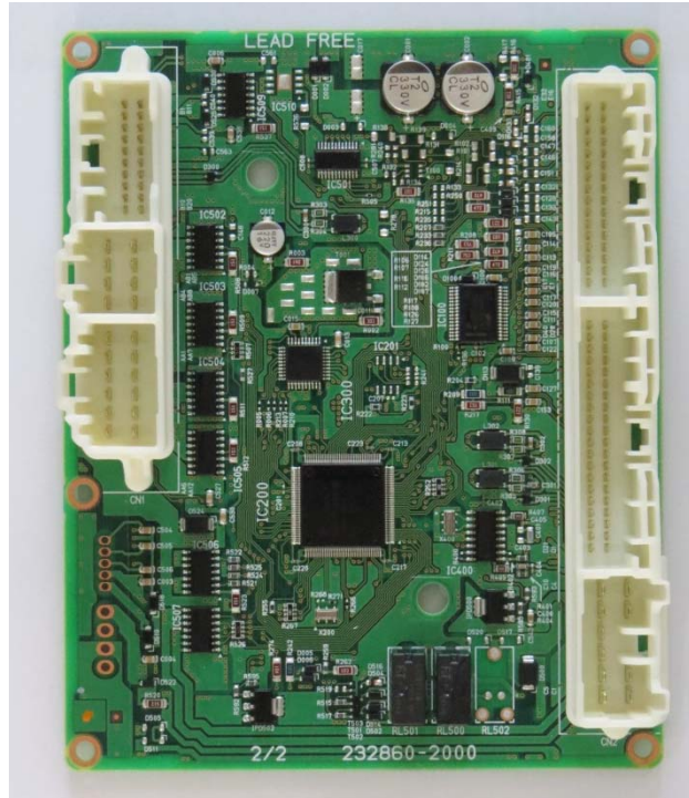
Component side
