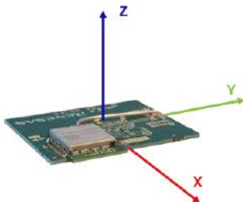
Figure 13. Measurement plane definition
