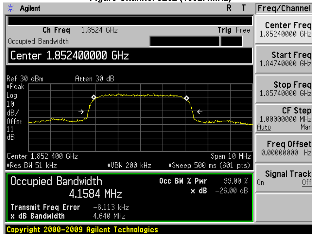
Figure Channel 9262 (1852.4MHz)
