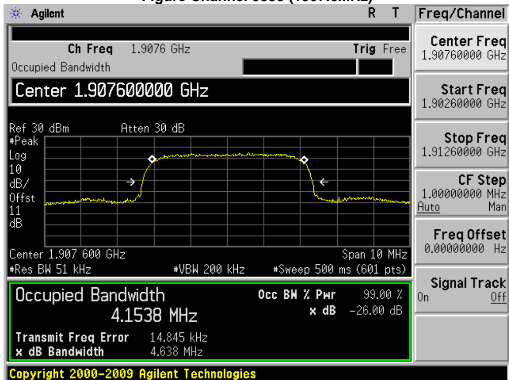
Figure Channel 9538 (1907.6MHz)
