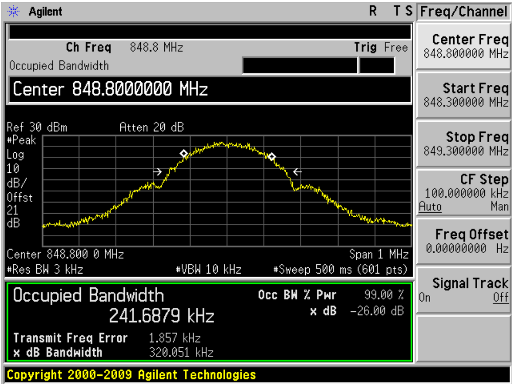
Figure Channel 251 (848.80MHz)
