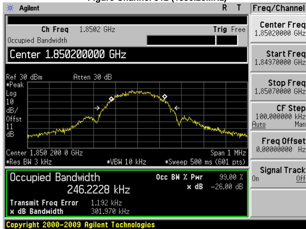
Figure Channel 512 (1850.20MHz)
