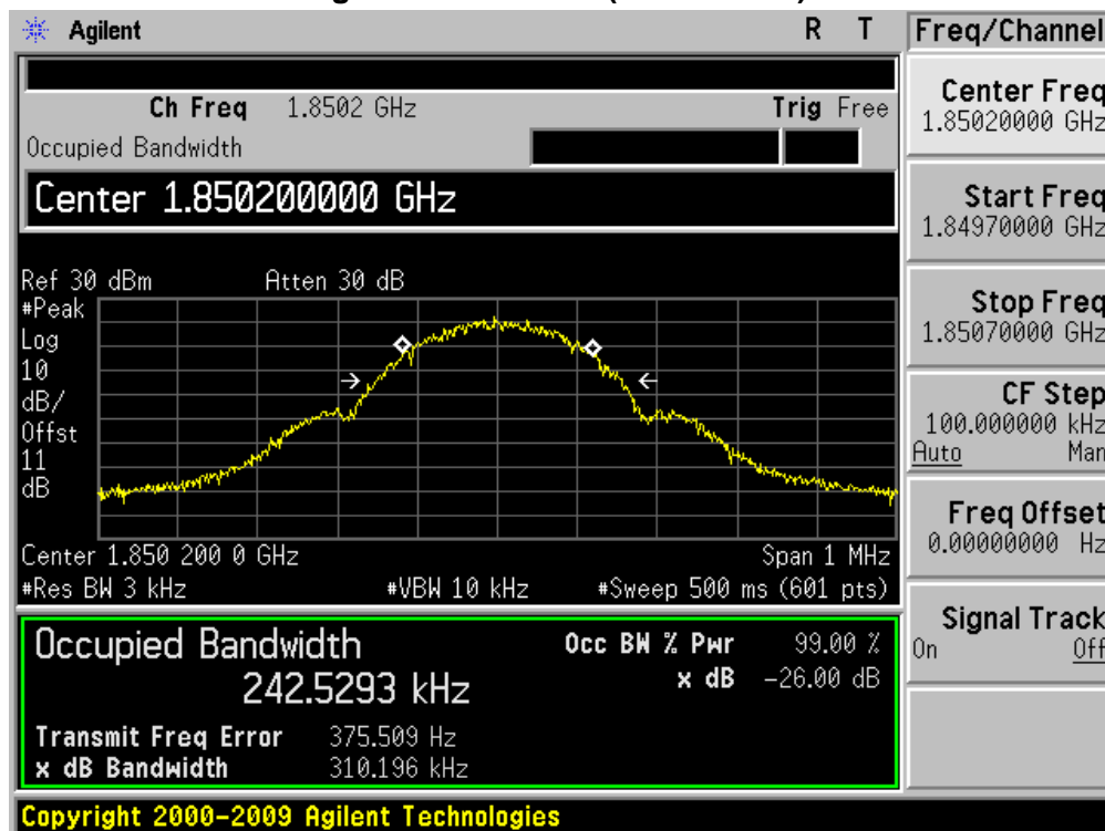
Figure Channel 512 (1850.20MHz)
