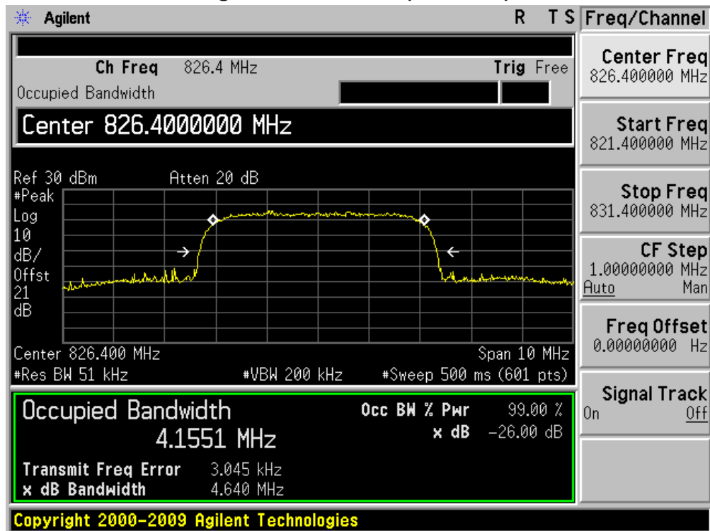
Figure Channel 4132 (826.4MHz)
