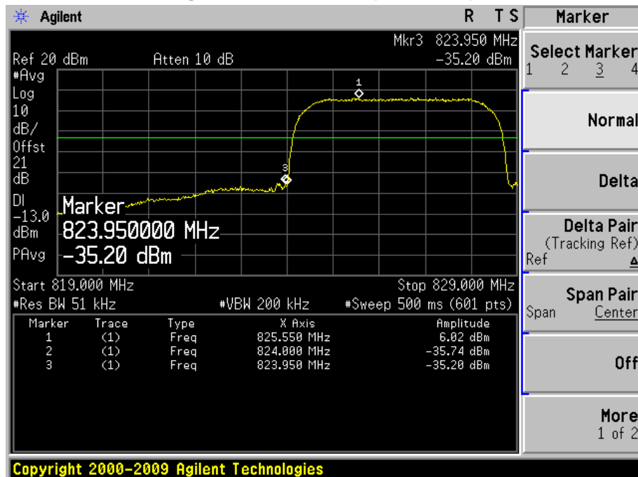
Figure Channel 4132 (826.4MHz)
