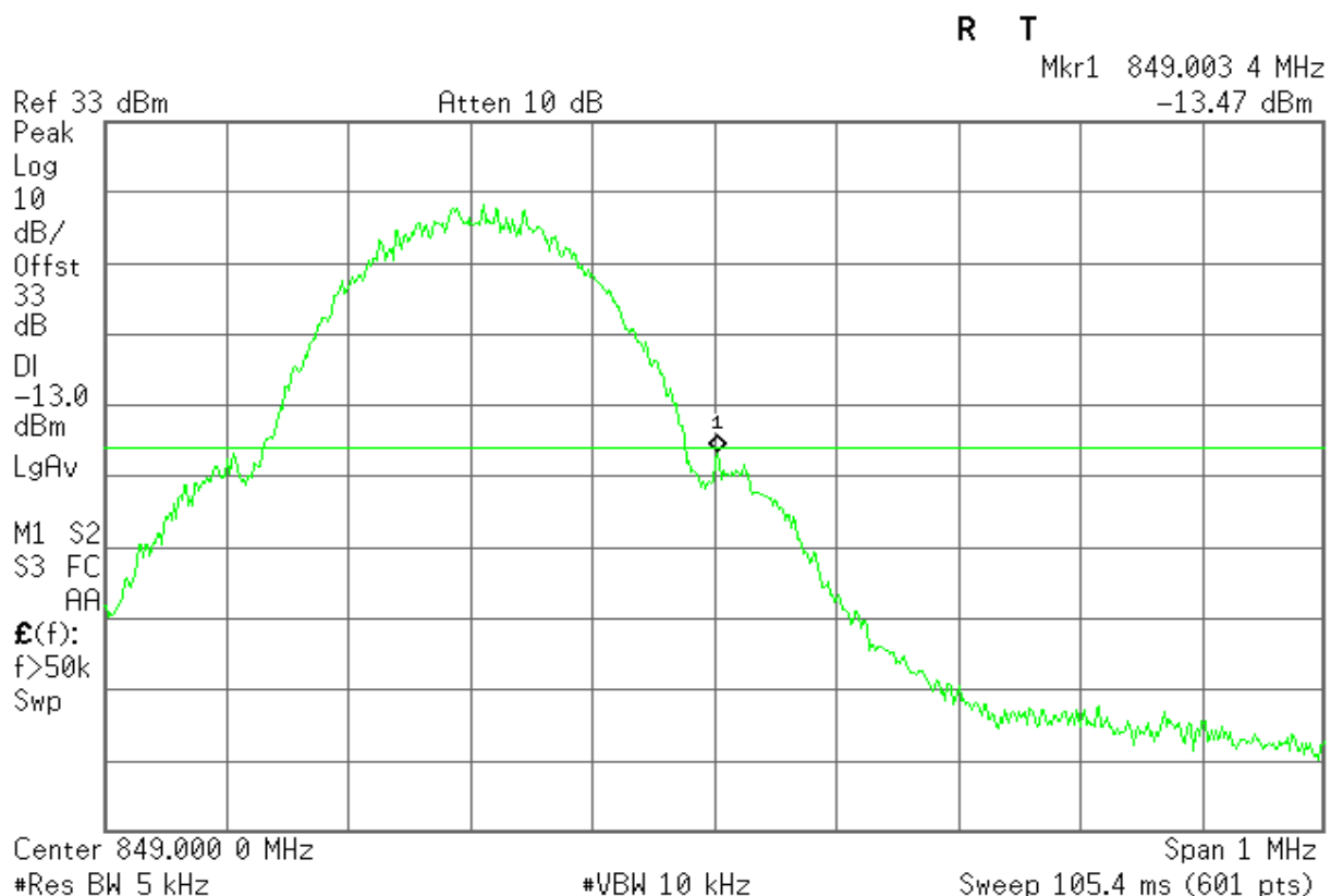
Figure 9-2: Band Edge emissions –GPRS CH High
