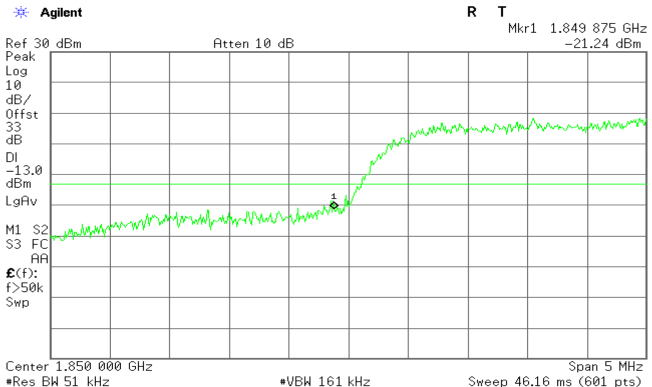
Figure 16-4: Band Edge emissions –WCDMA CH Low
