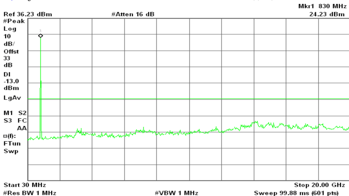
Figure 11-2: Out of Band emission at antenna terminals – WCDMA CH Mid
