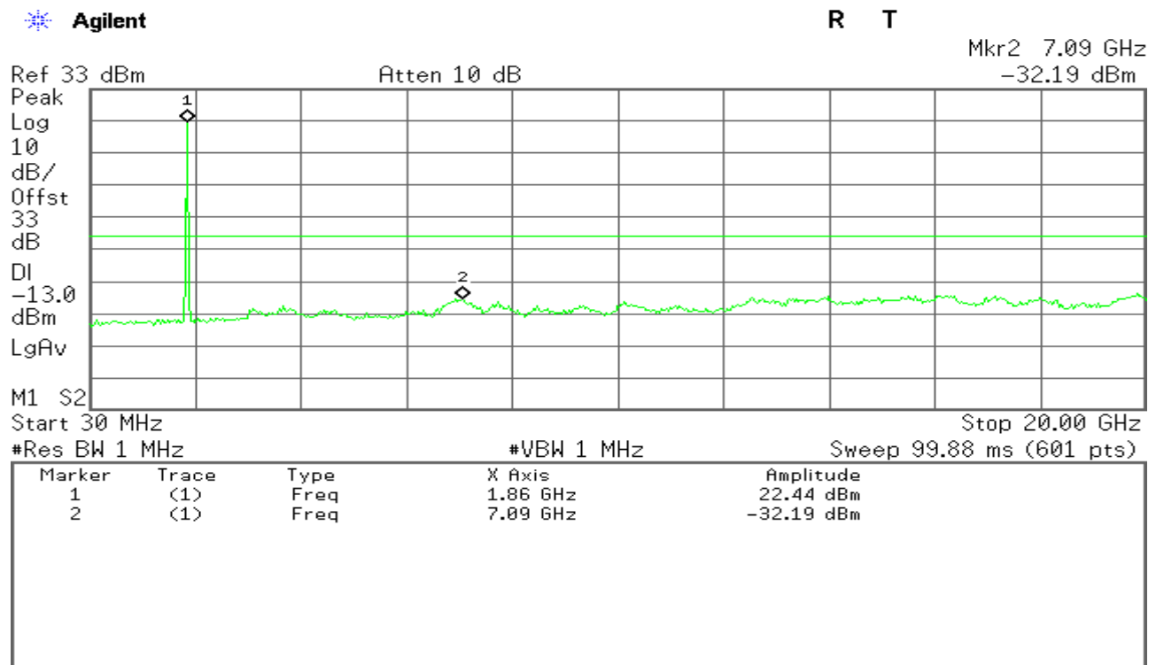
Figure 16-1: Out of Band emission at antenna terminals – WCDMA CH Low
