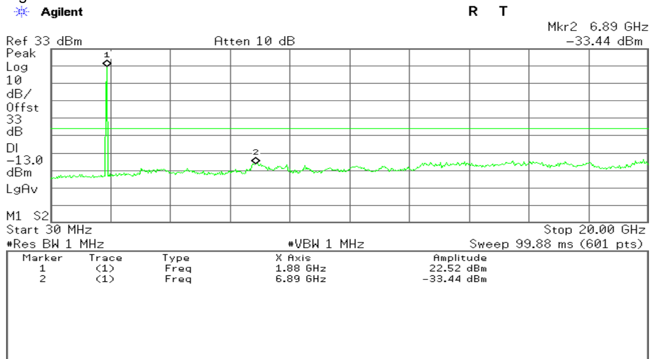
Figure 16-2: Out of Band emission at antenna terminals – WCDMA CH Mid
