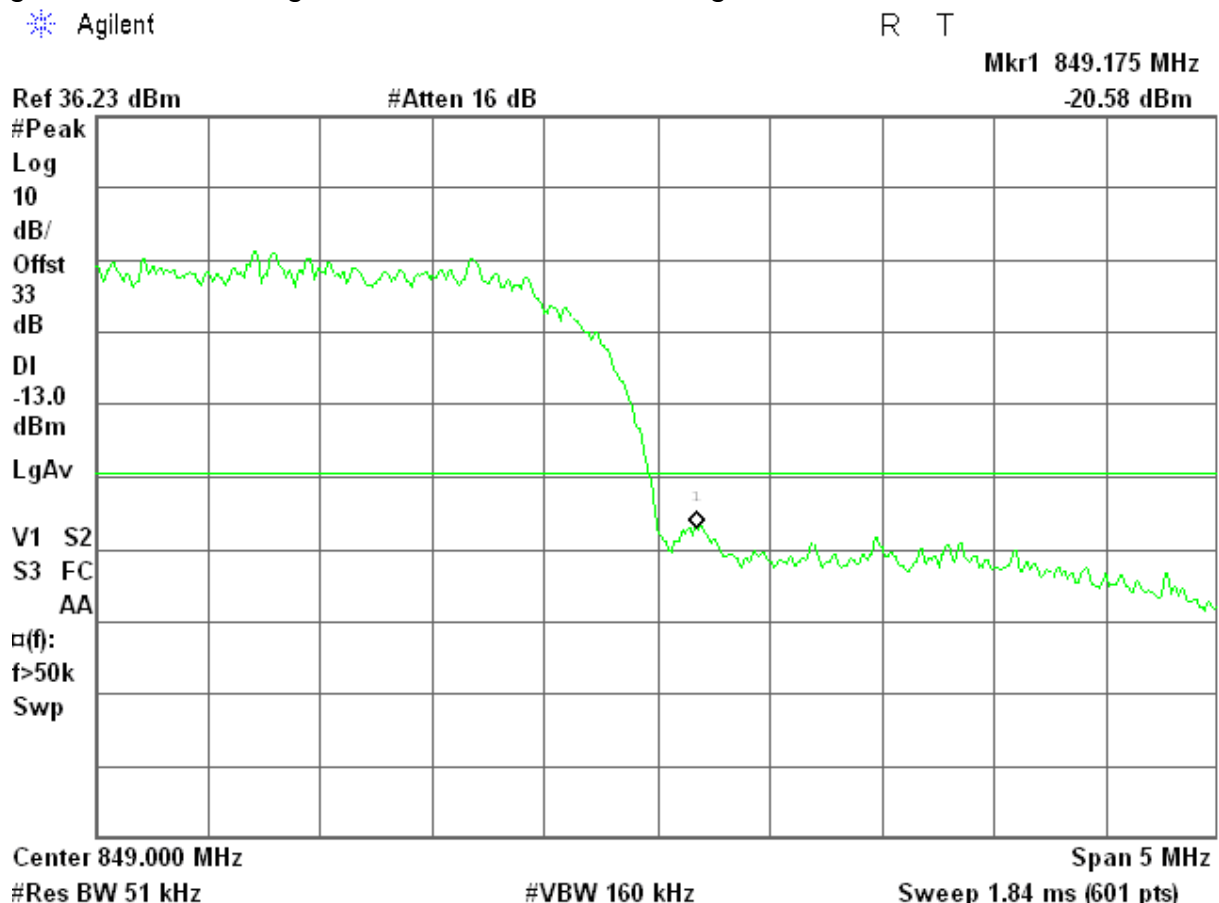
Figure 12-5: Band Edge emissions – HSDPA CH High
