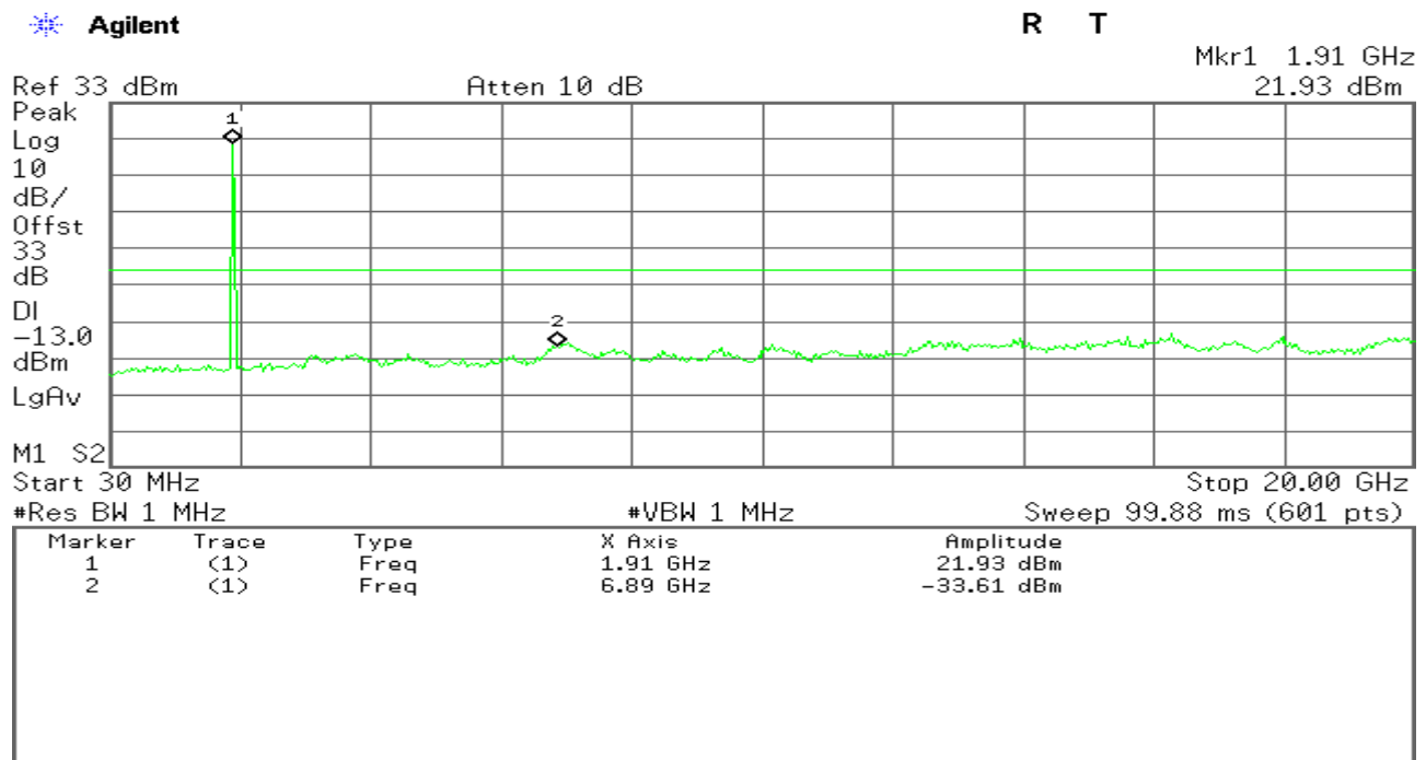
Figure 16-3: Out of Band emission at antenna terminals – WCDMA CH High
