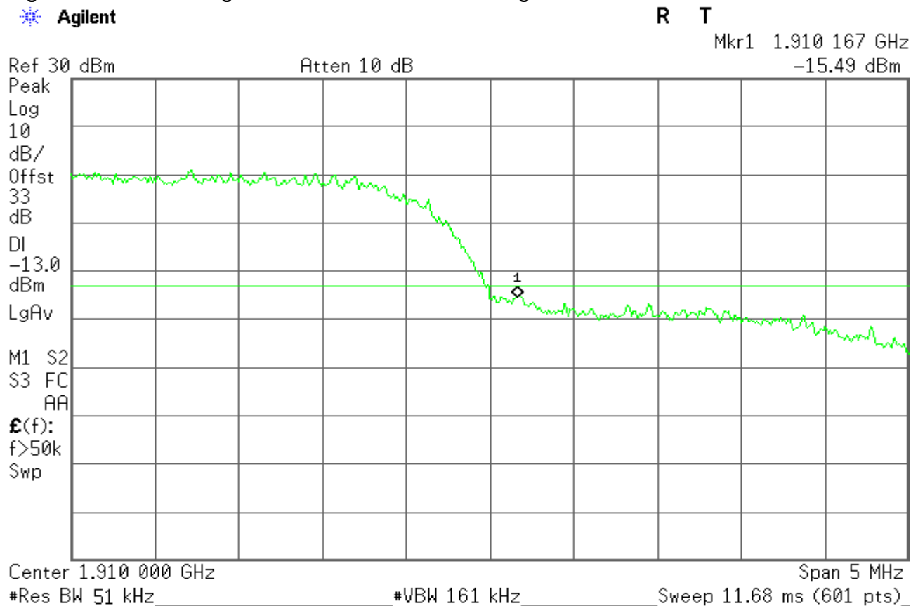
Figure 17-5: Band Edge emissions – HSDPA CH High
