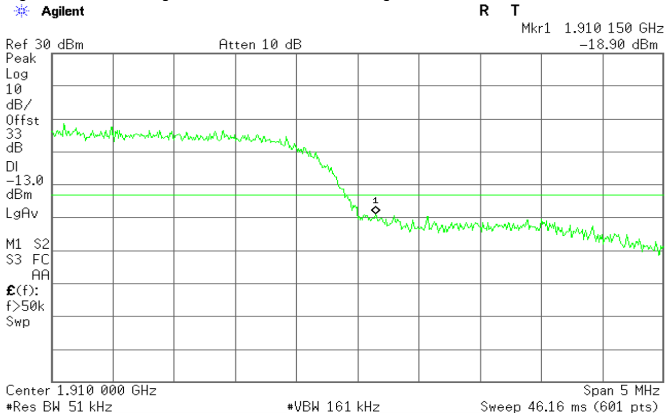
Figure 16-5: Band Edge emissions –WCDMA CH High
