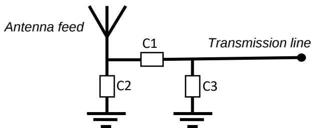
Matching circuit
