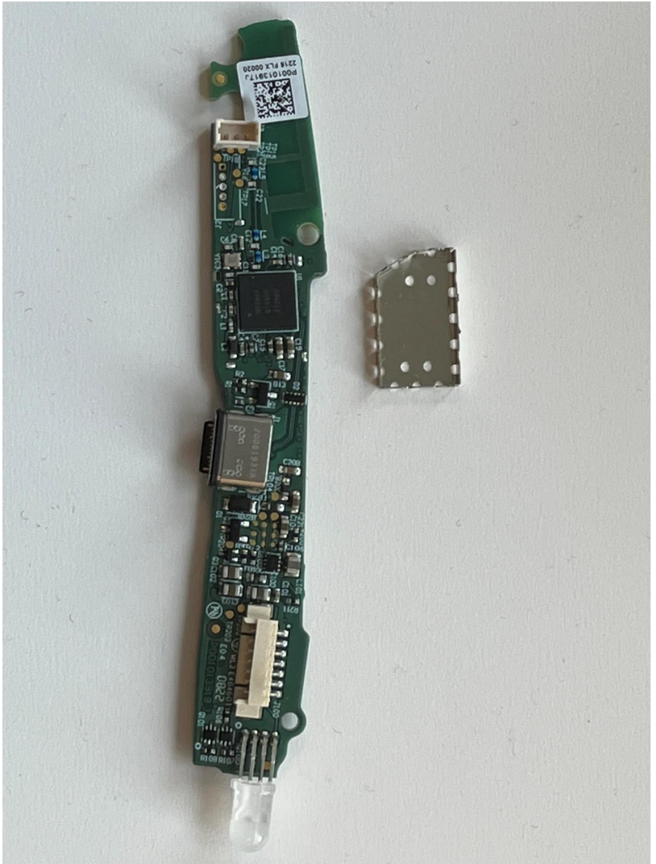
PCB front side without metal shielding
