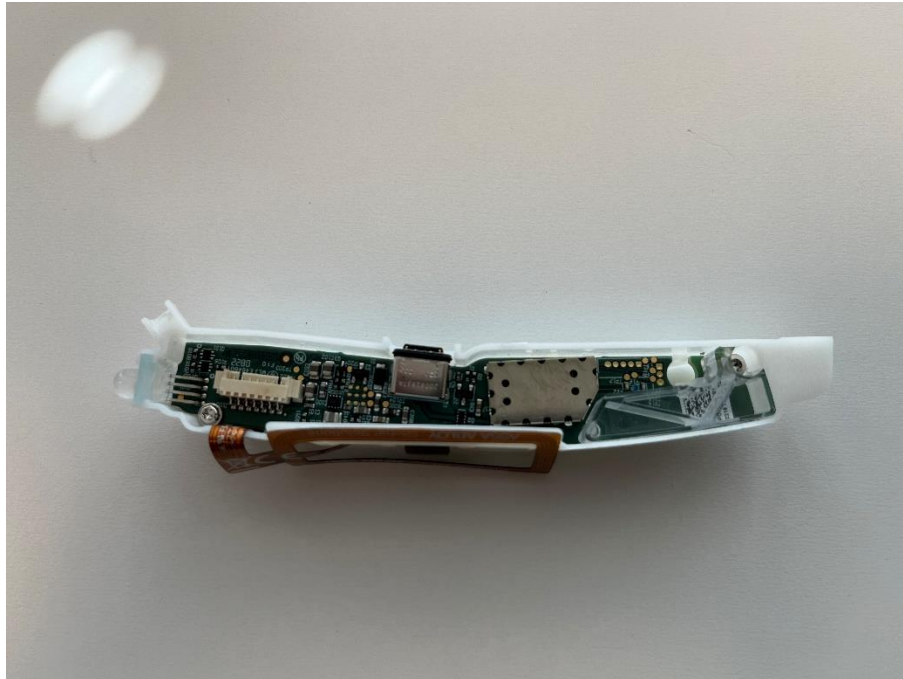
Top view of the RCC 1601 module before potting
