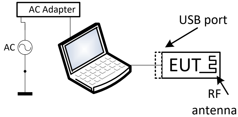
Figure 3.6-1: Setup diagram
