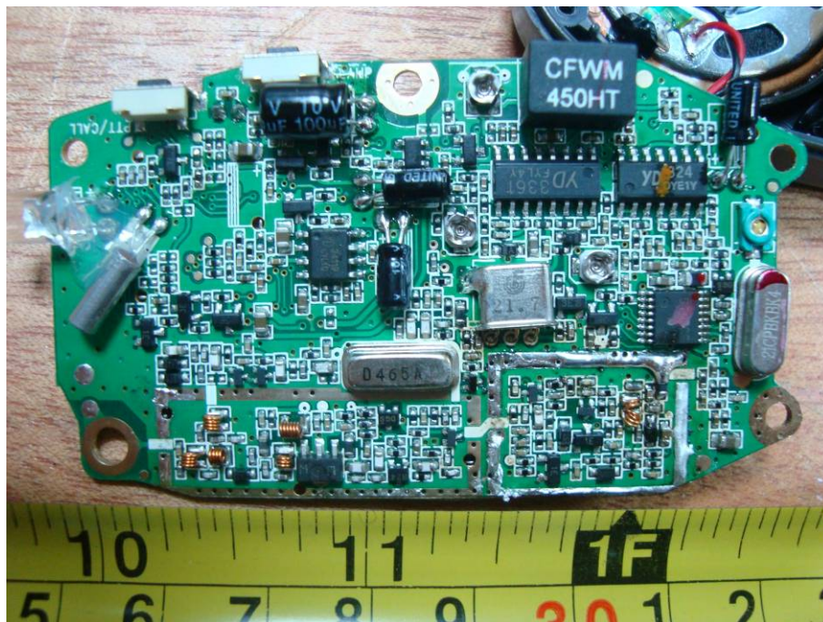
EUT- Main Board without RF Module Metal Cover Top View
