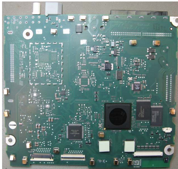
Figure11: VP2 main board PCB bottom view
