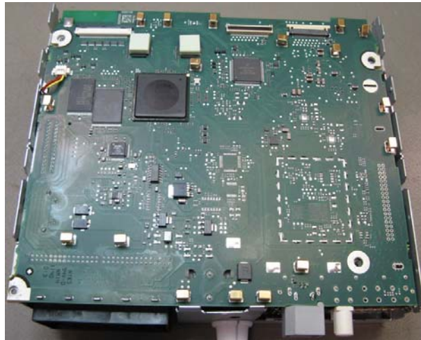
Figure9: VP2 bottom view without front unit
