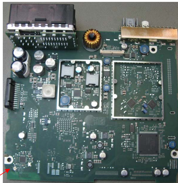
Figure12: VP2 main board PCB top view
