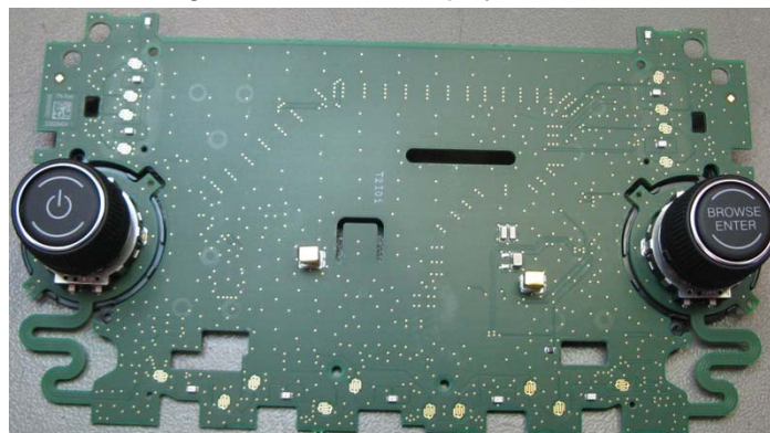
Figure17: VP2 front PCB top view
