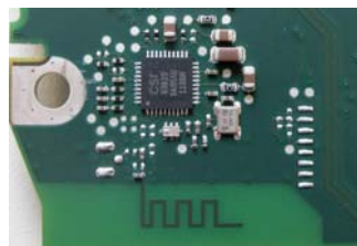
Figure13: VP2 Bluetooth module with PCB antenna
