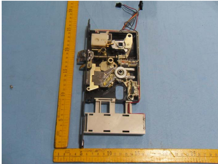
Figure 5 Part of the EUT-Inside View
