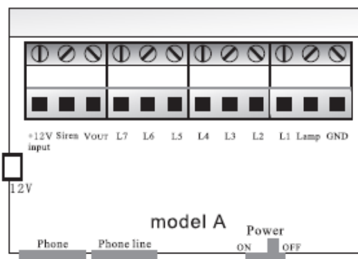
Figure 3: The back view of the panel
