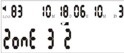
Figure 25: Detector No 2 in zone 3 is low voltage
