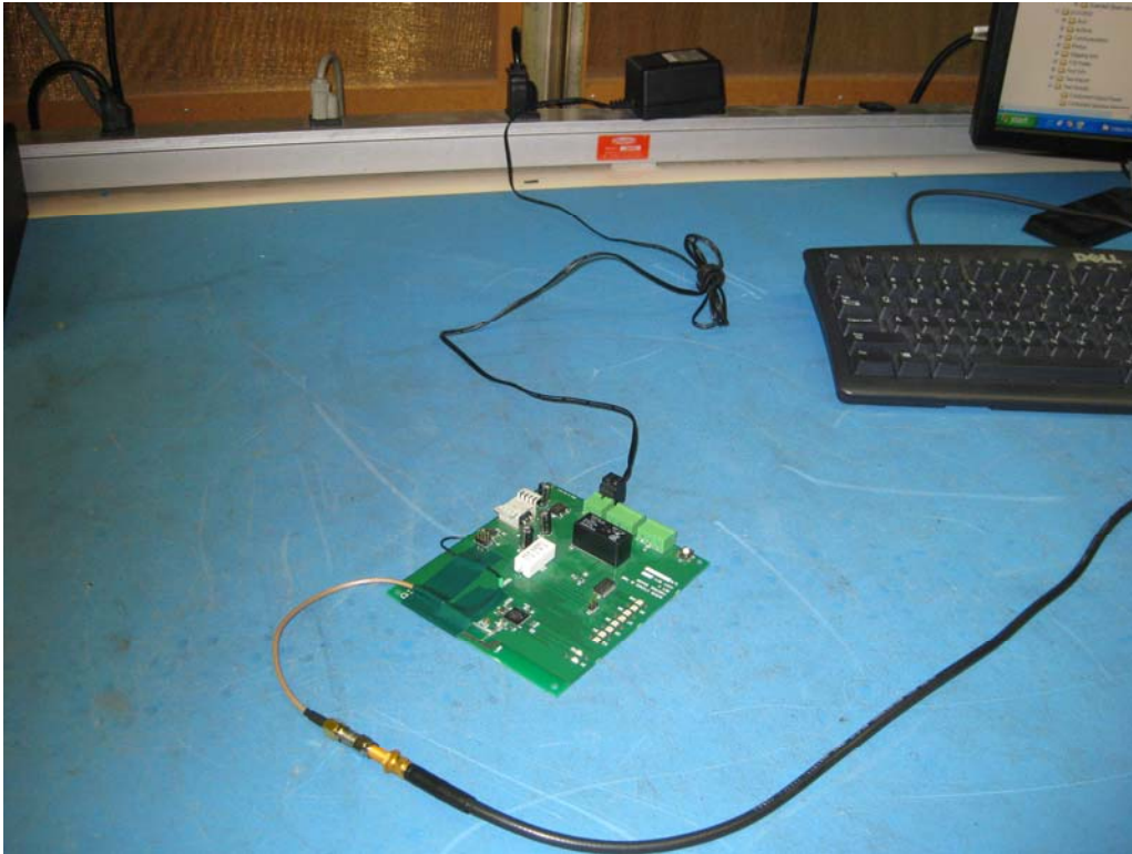
RF Conducted #2
