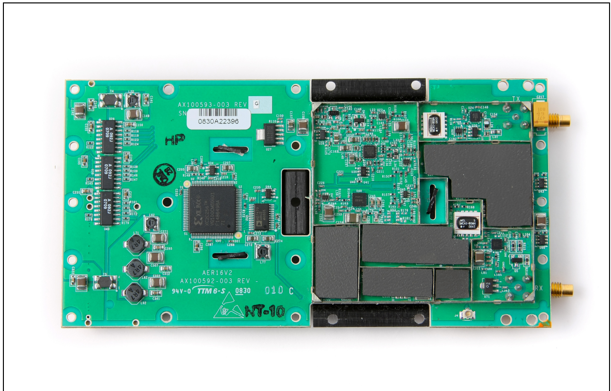
Figure 5: Modem – Front without Shields
