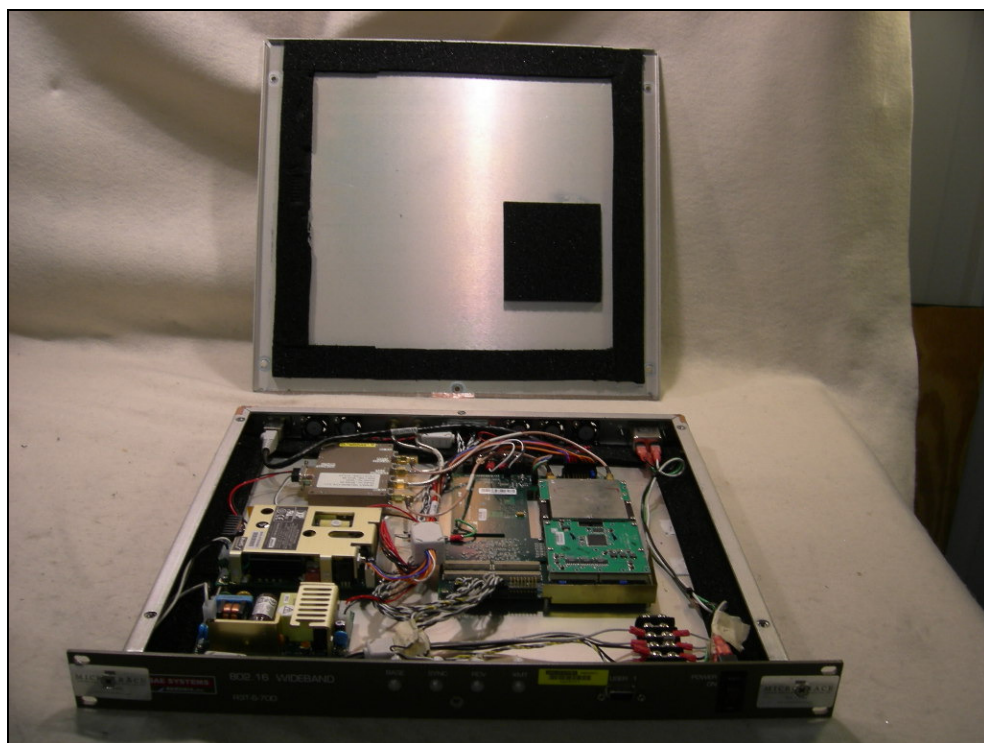
Figure 6: Indoor Unit Assembled
