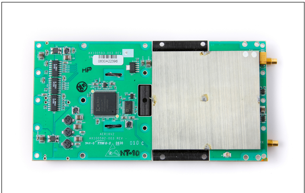
Figure 4: Modem – Front with Shields
