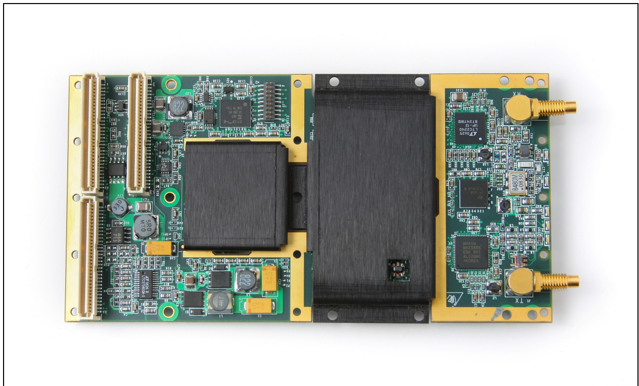
Figure 3: Modem - Back
