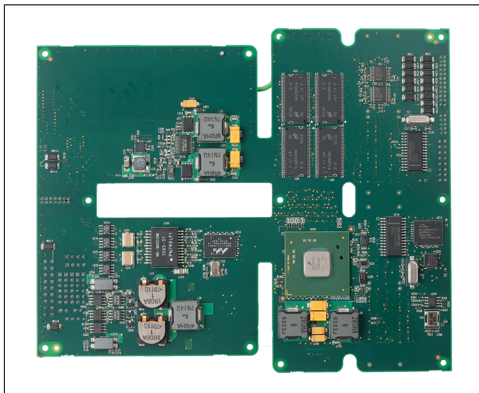
Figure 2: Motherboard - Bottom
