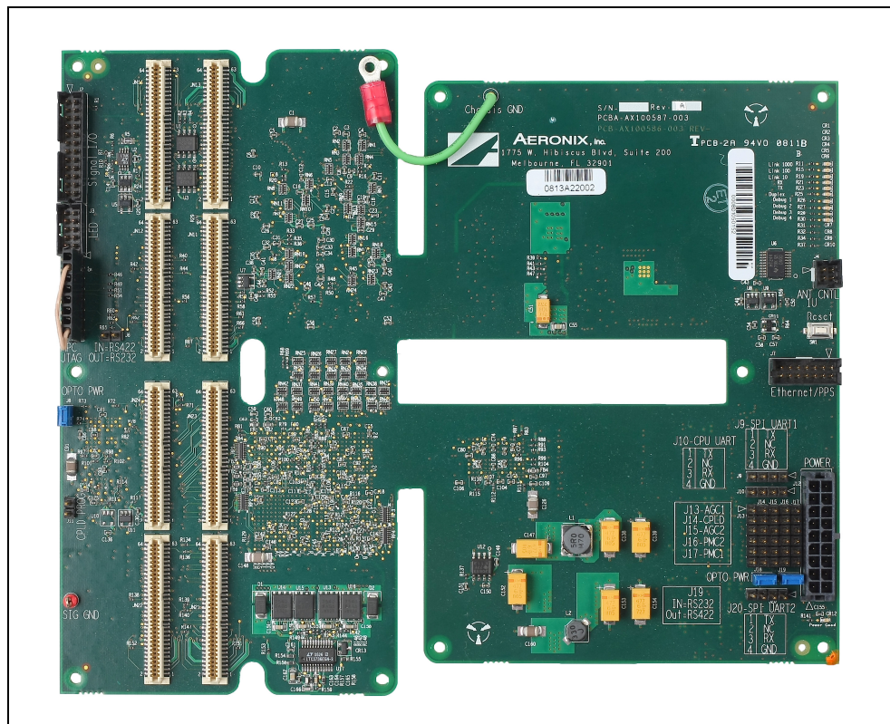
Figure 1: Motherboard – Top
