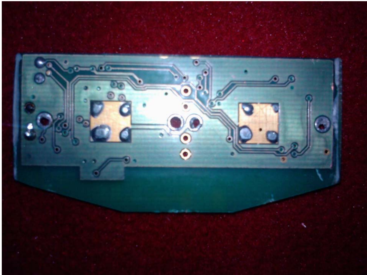
EUT – Circuit Board, Bottom without battery cover
