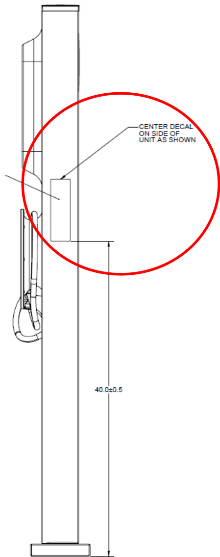
Pedestal Product Label Position (Not To Scale)
