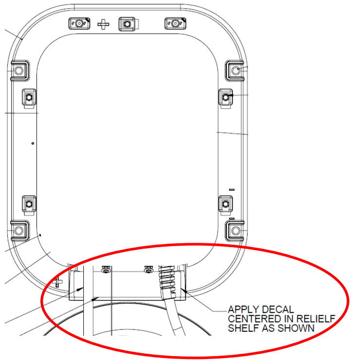
Wall Mount Product Label Position (Not To Scale)
