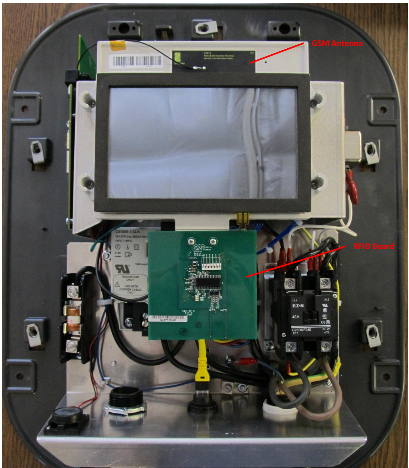
Figure 1 - EVSE Front View
