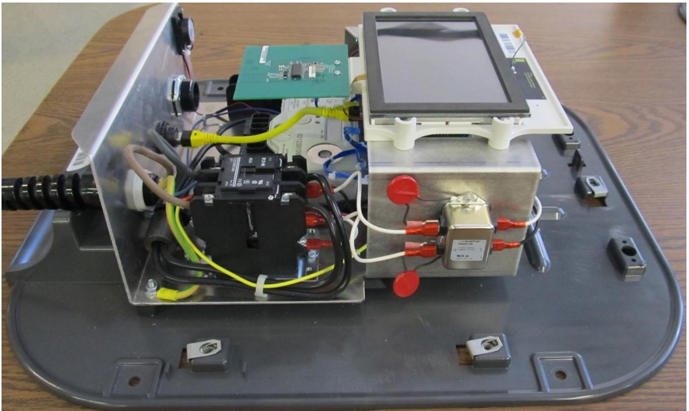
Figure 2 - EVSE Right View
