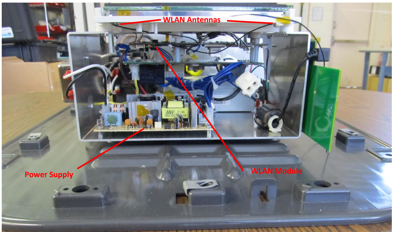
Figure 6 - EVSE Top View
