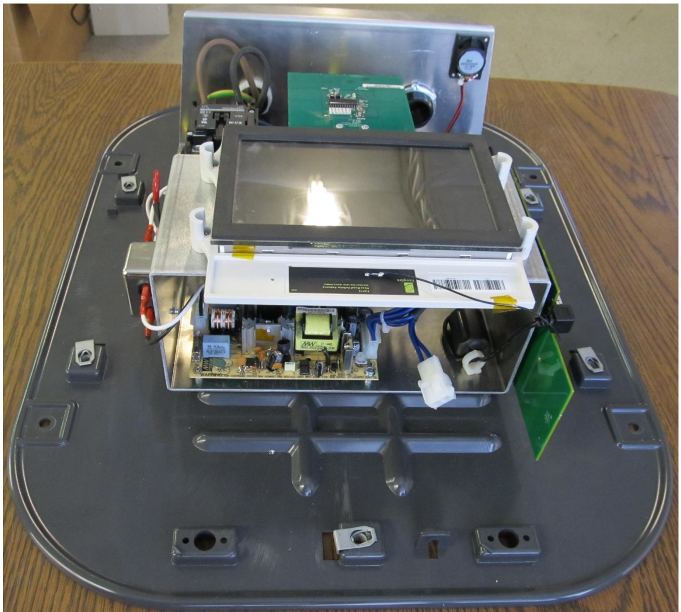
Figure 5 - EVSE Top View
