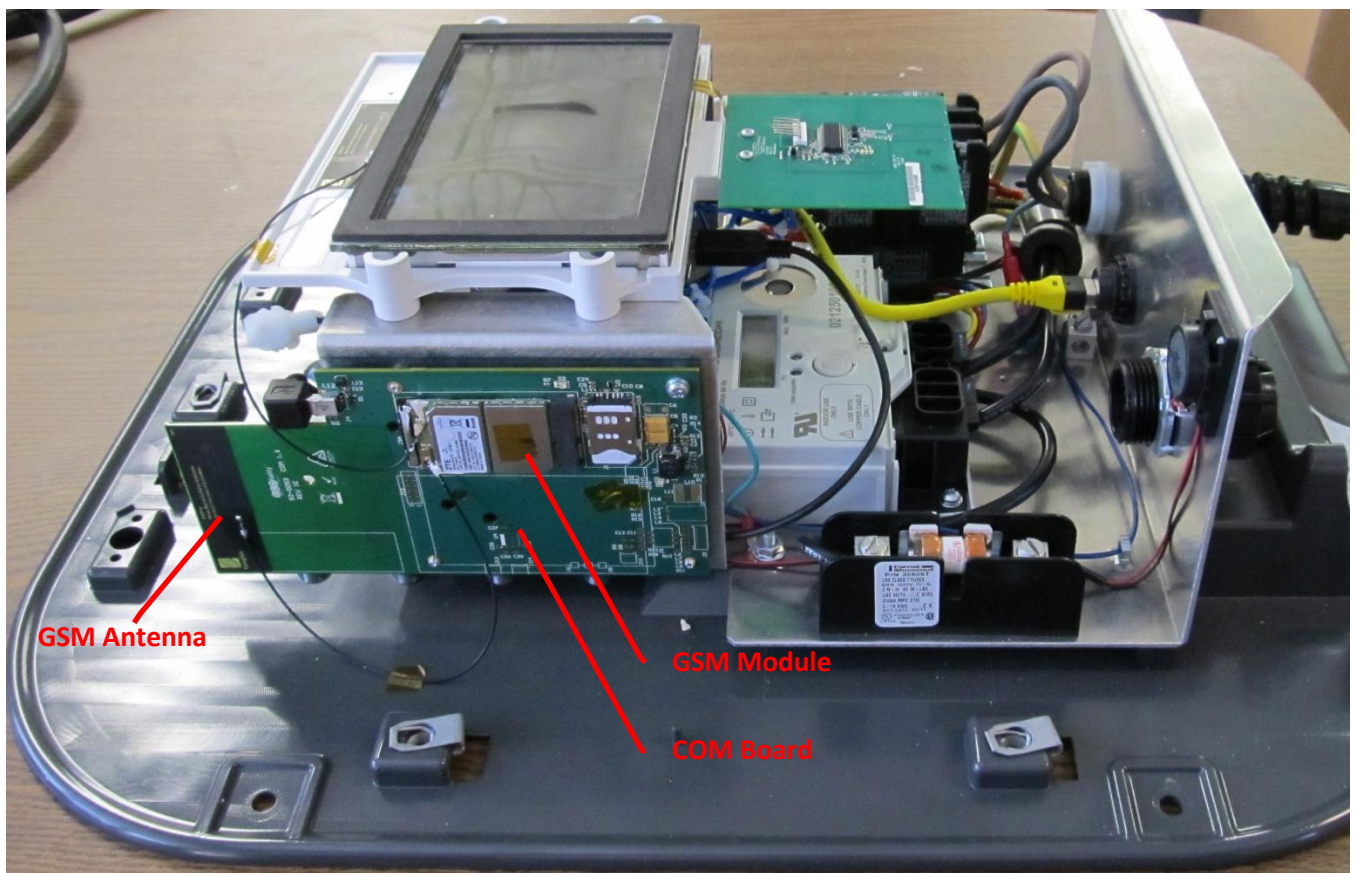
Figure 3 - EVSE Left View
