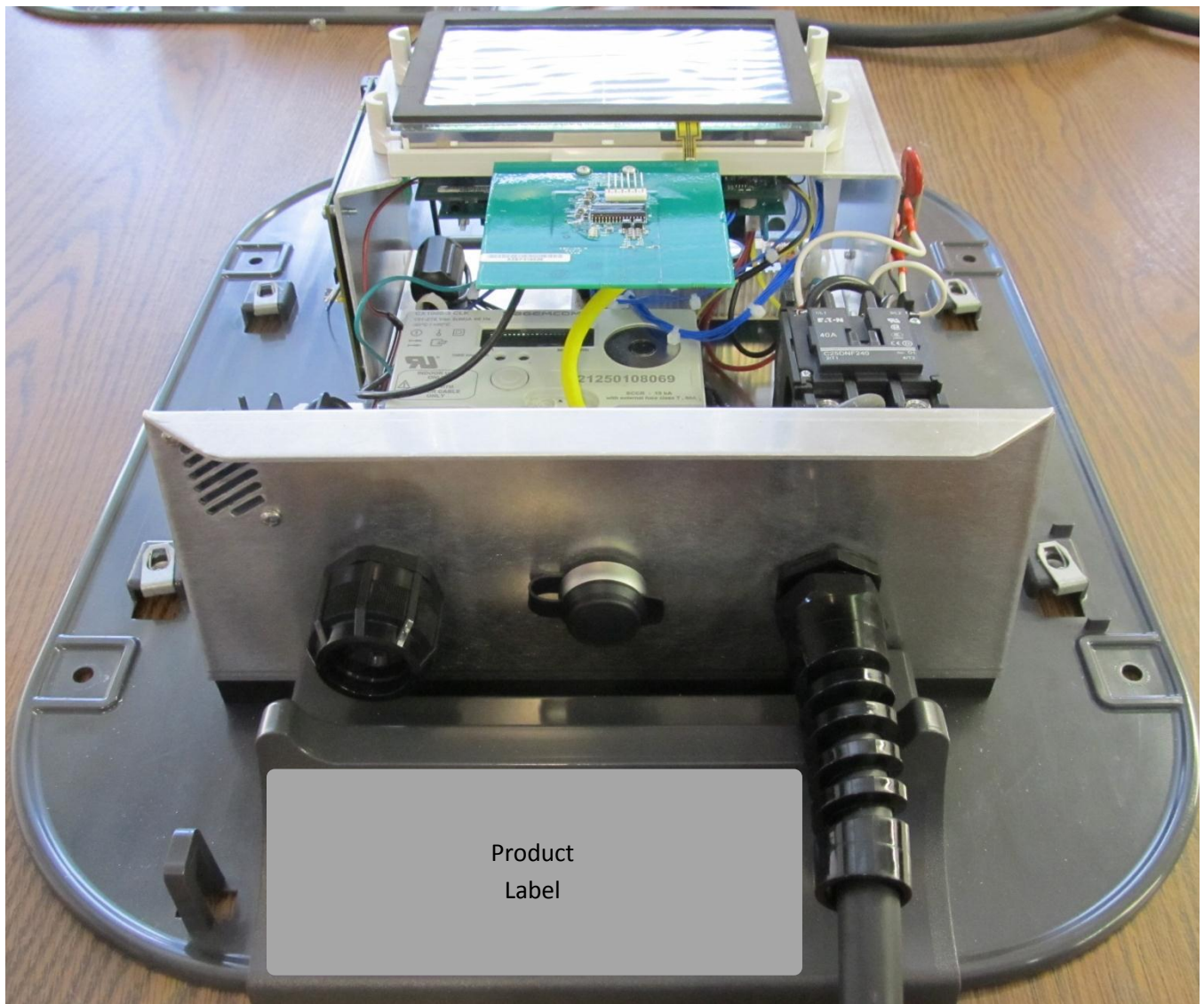
Figure 4 - EVSE Bottom View
