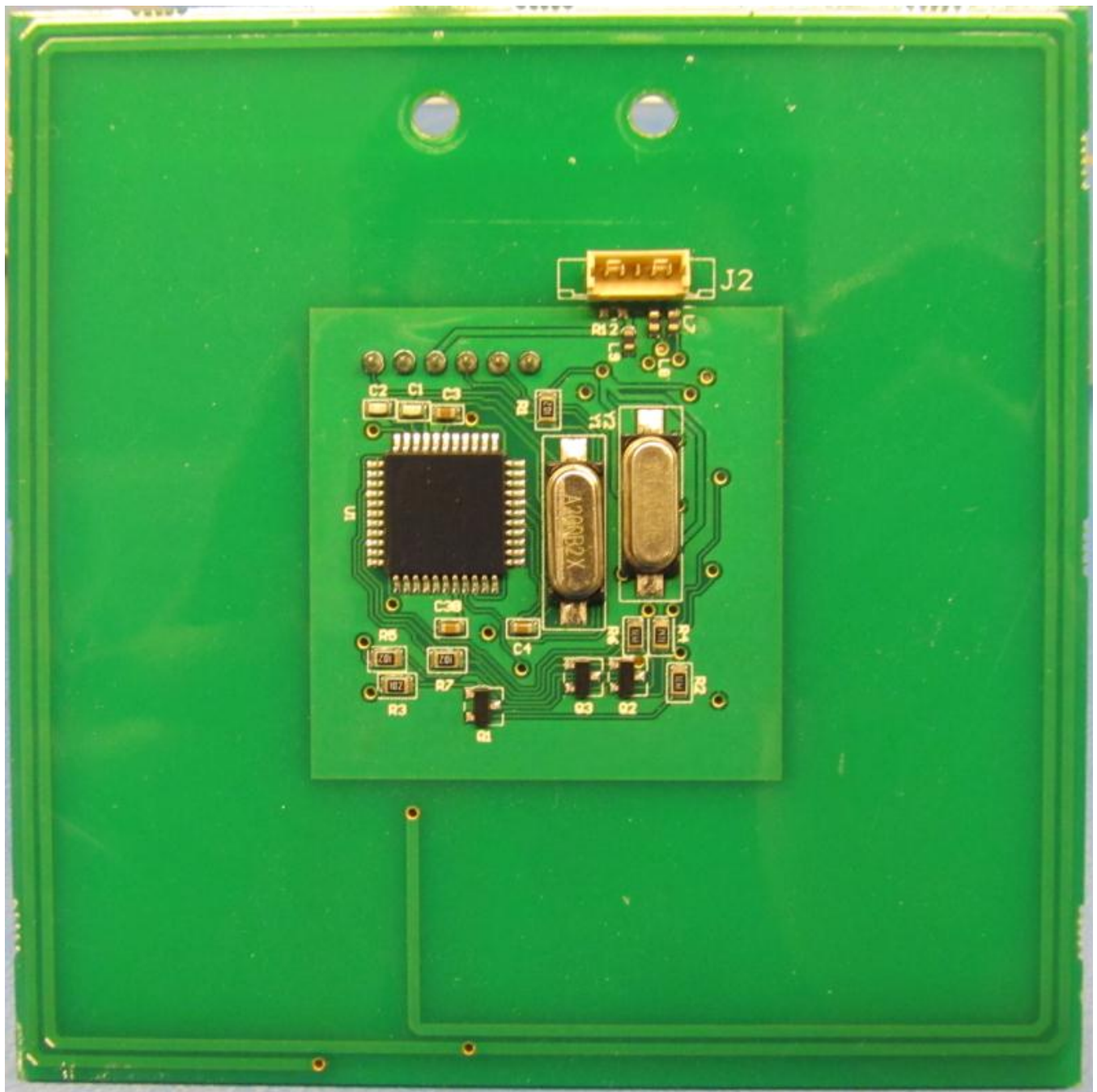
Figure 2 - RFID Board Back View
