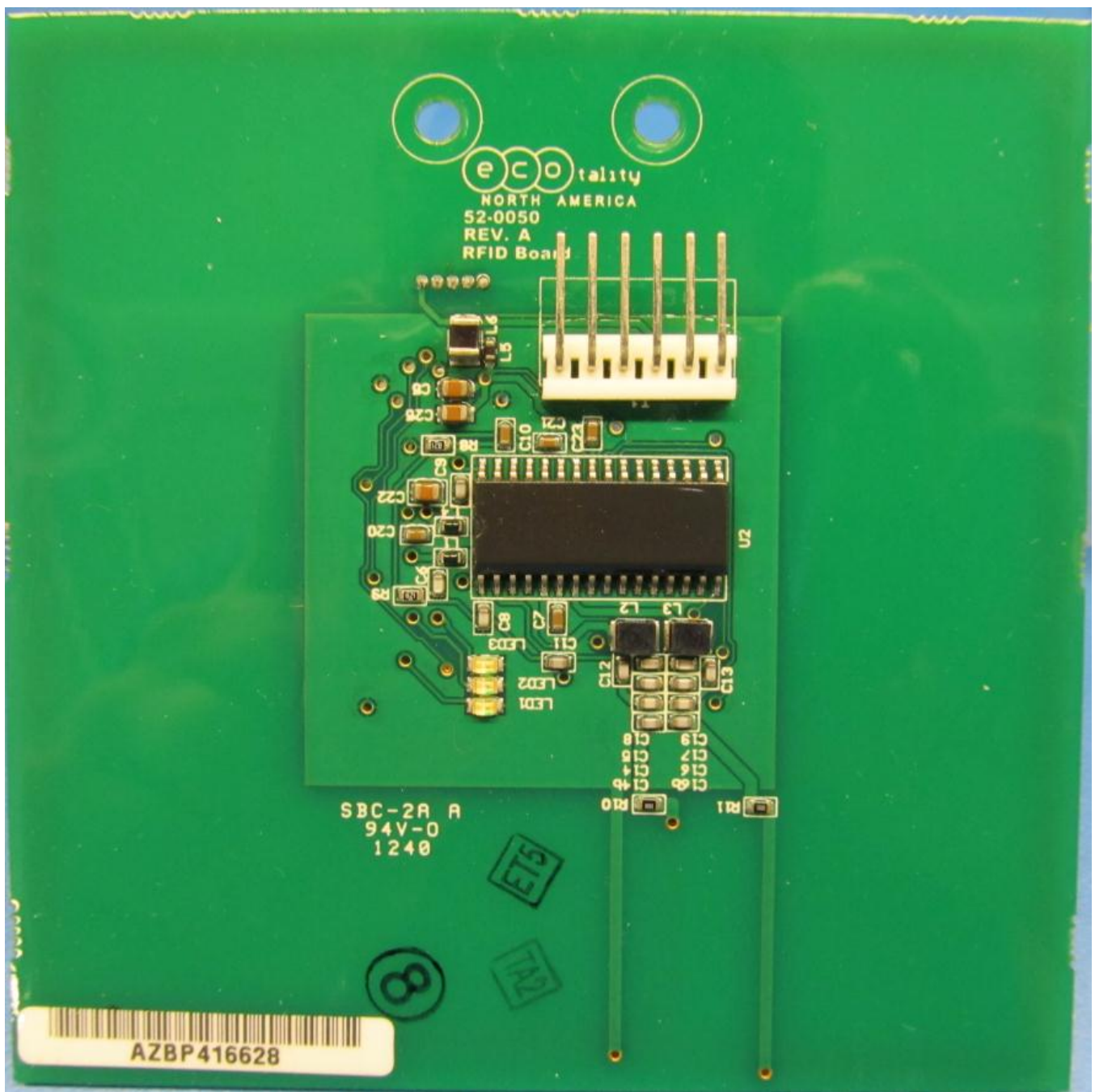
Figure 1 - RFID Board Front View
