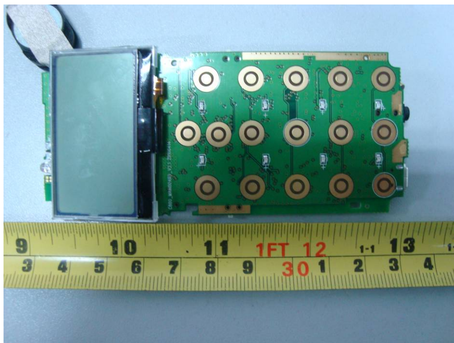
EUT – Main Board with Keyboard Cover Off Top View
