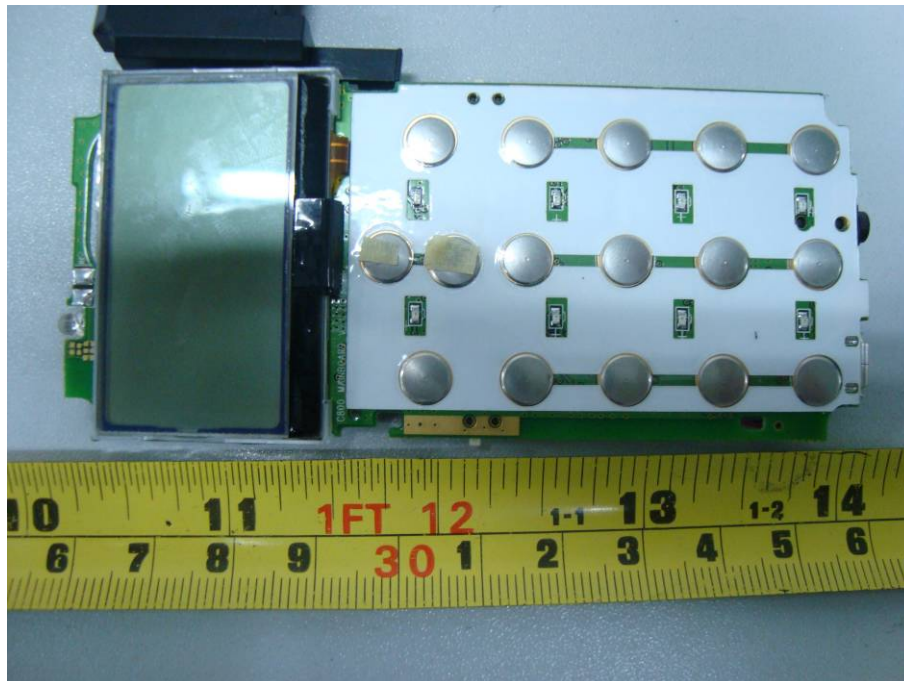
EUT – Main Board with LCD and Keyboard Top View
