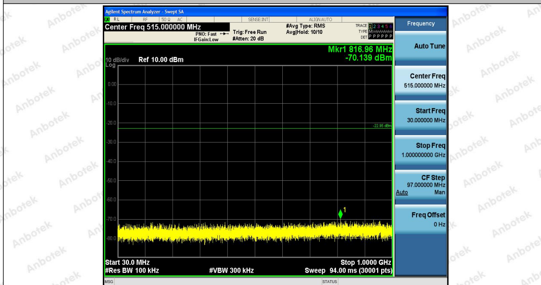
2.4G_Ant1_2440_30~1000
