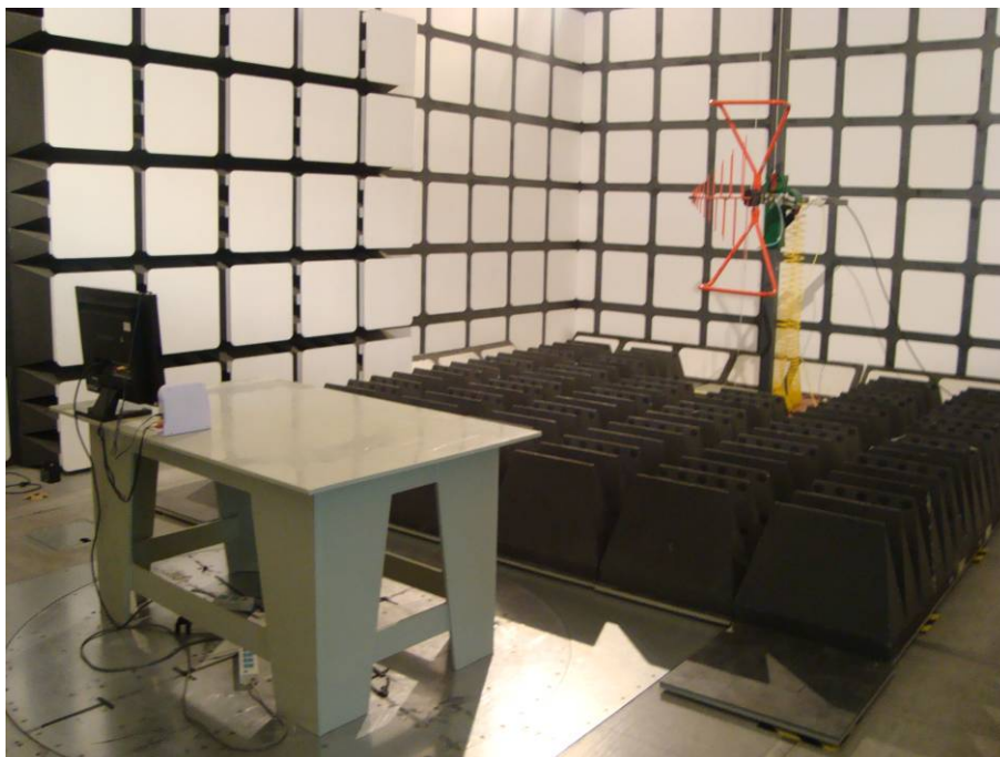
Below 1 GHz: Spurious Radiated Emissions with Battery - Rear View
