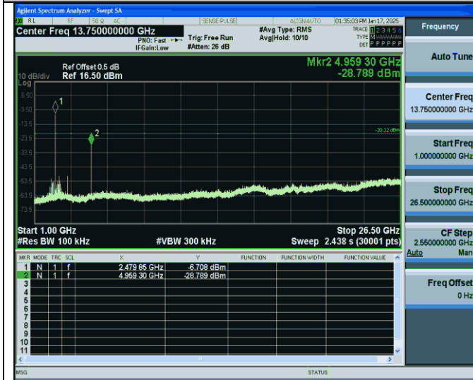
3DH5-Ant1-2480-1000~26500-PASS
