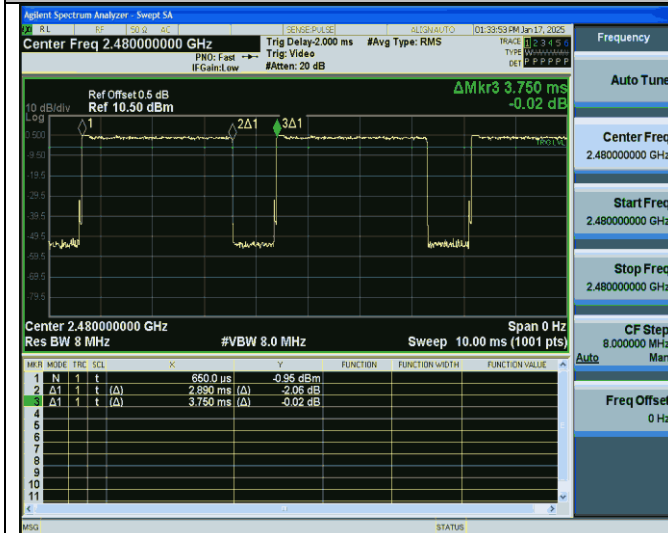
NTNV-3DH5-Ant1-2480
