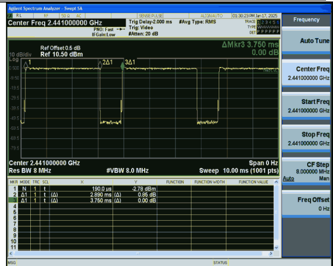
NTNV-3DH5-Ant1-2441
