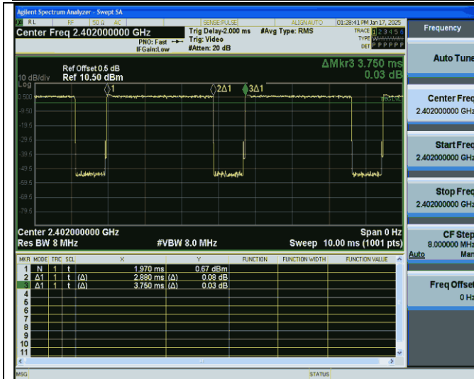
NTNV-3DH5-Ant1-2402
