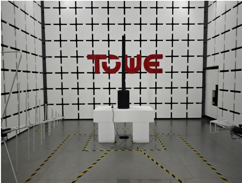
Radiated Spurious Emissions (30MHz to 1000MHz)
