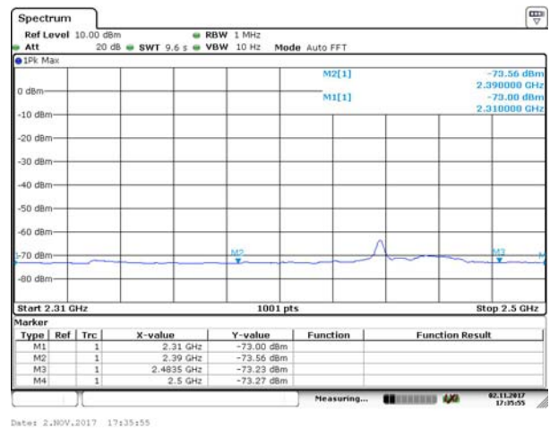
2441MHz - Average
