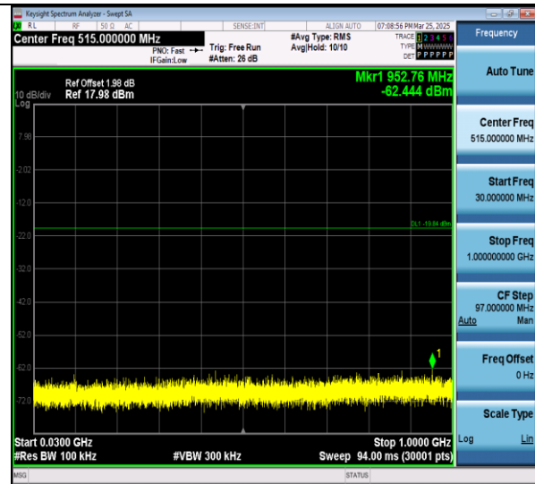
BLE_1M-Ant1-2480-30~1000-PASS
