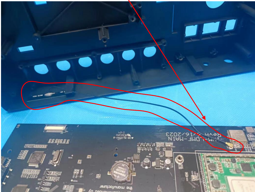
View of BT & WIFI antenna
