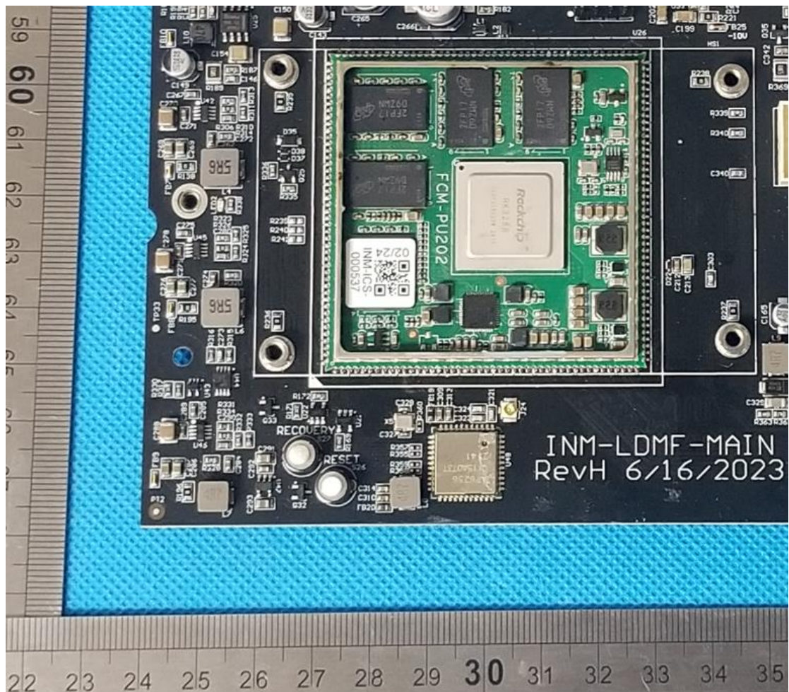
Inner circuit top view
