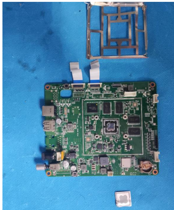
Inner circuit bottom view
