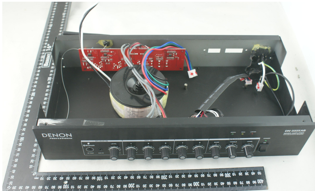
EUT UNCOVER VIEW 4
