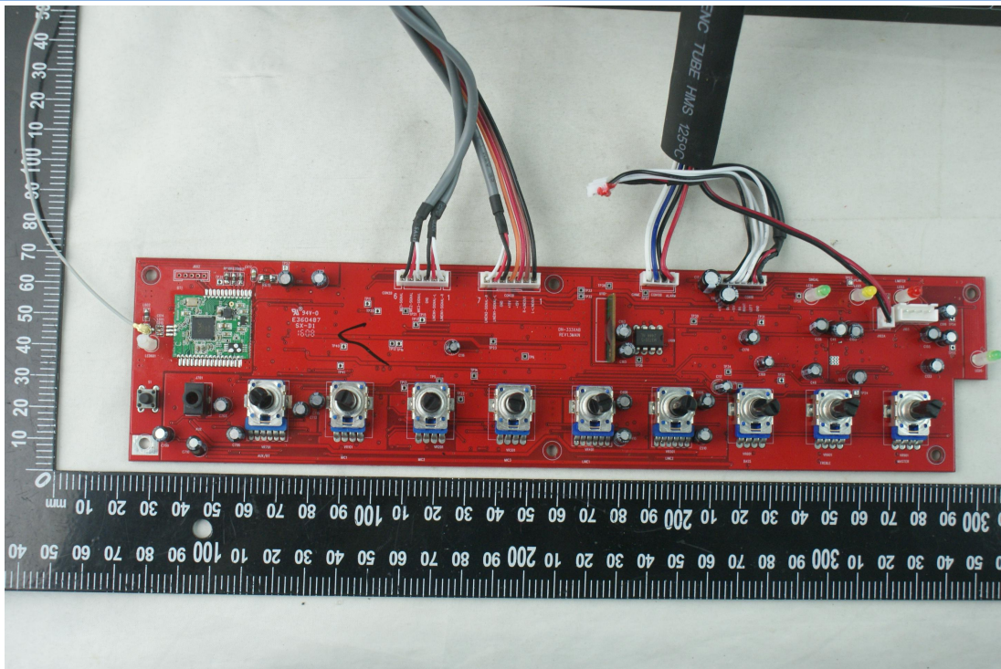
EUT MAIN BOARD FRONT VIEW 1
