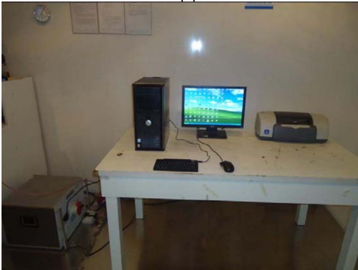
Conducted emission test setup photo
