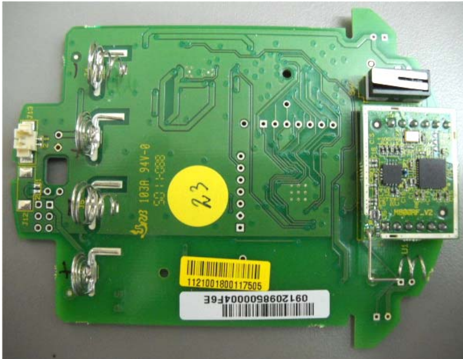
Photograph No.2 M800SRN indoor siren PCB front view
