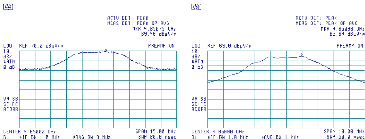
Plot 7.3.16 Radiated emission measurements at the third harmonic of carrier frequency
