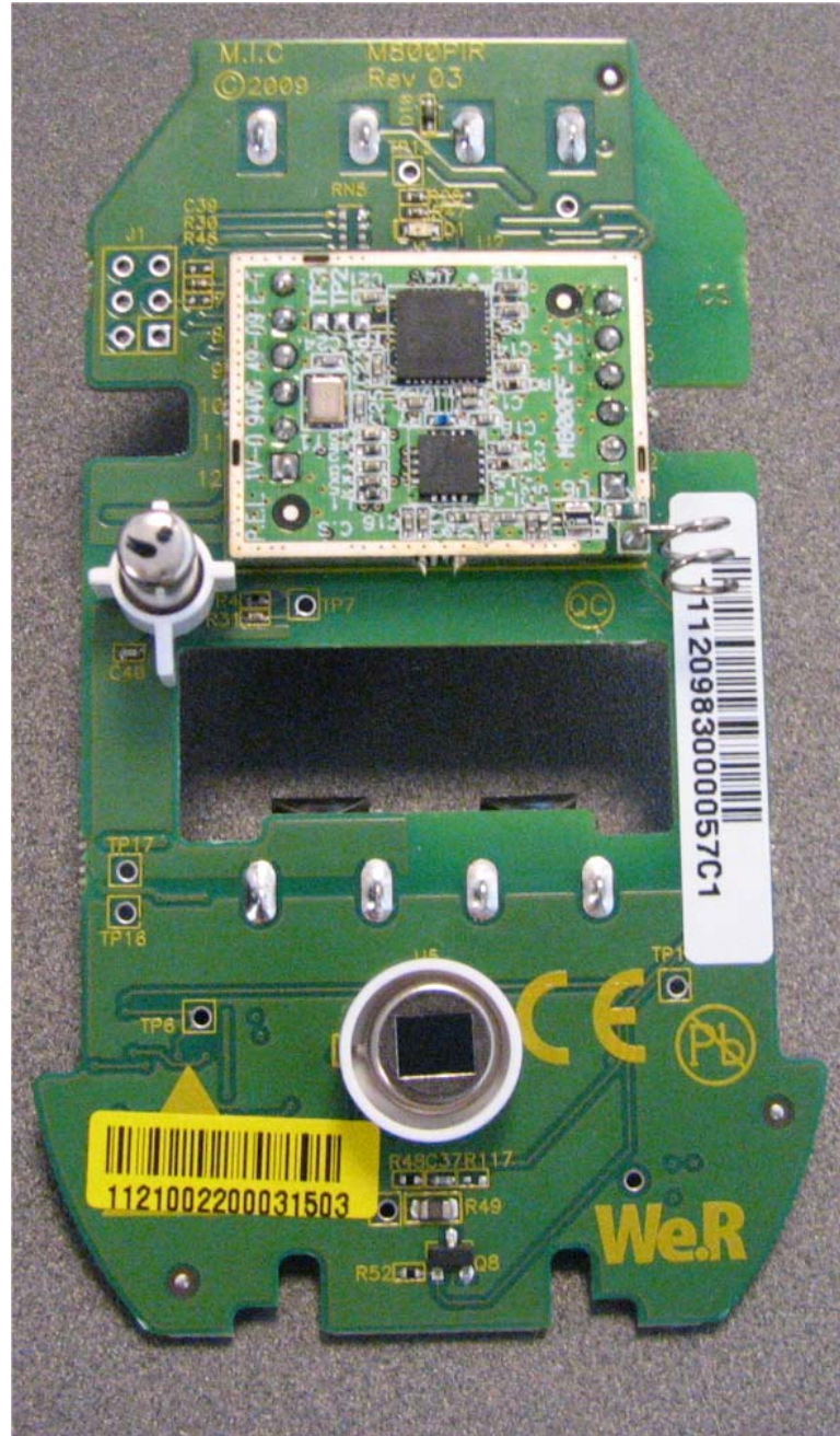
Photograph No.3 M800PIR motion detector PCB front view
