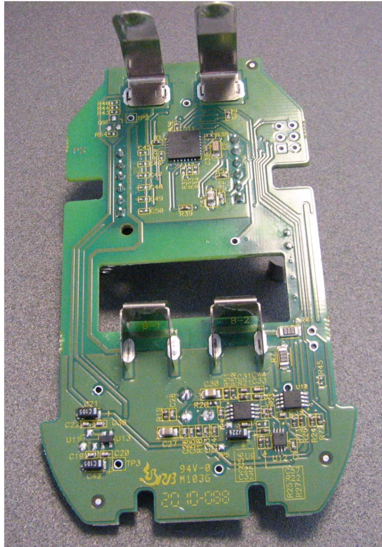
Photograph No.4 M800PIR motion detector PCB second side view
