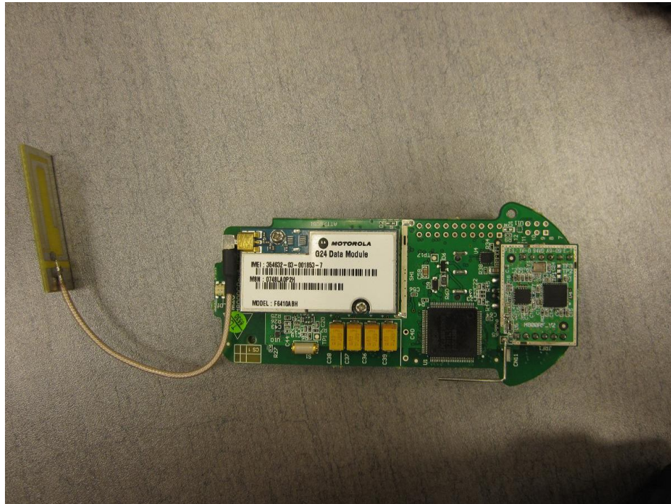
Front view of the board.
