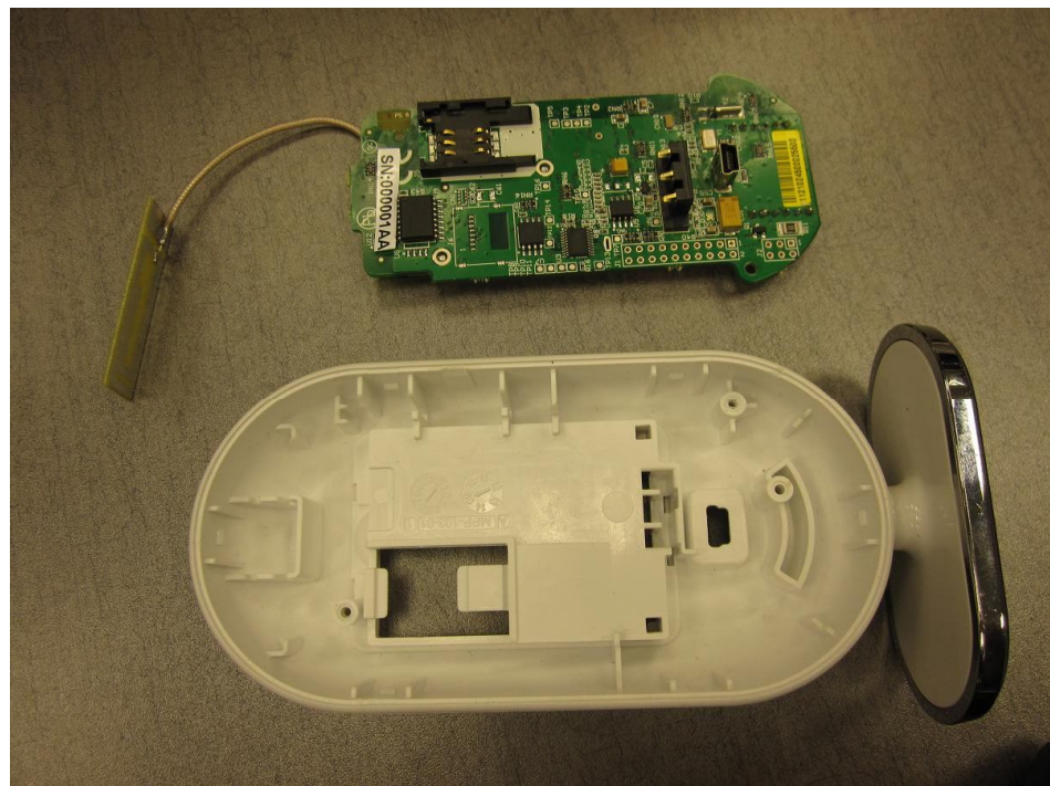
Internal view outside the enclosure.
