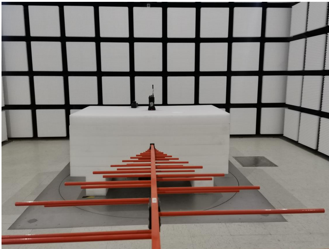
Radiated Emission Below 1GHz View-Model: DR7610S-1
