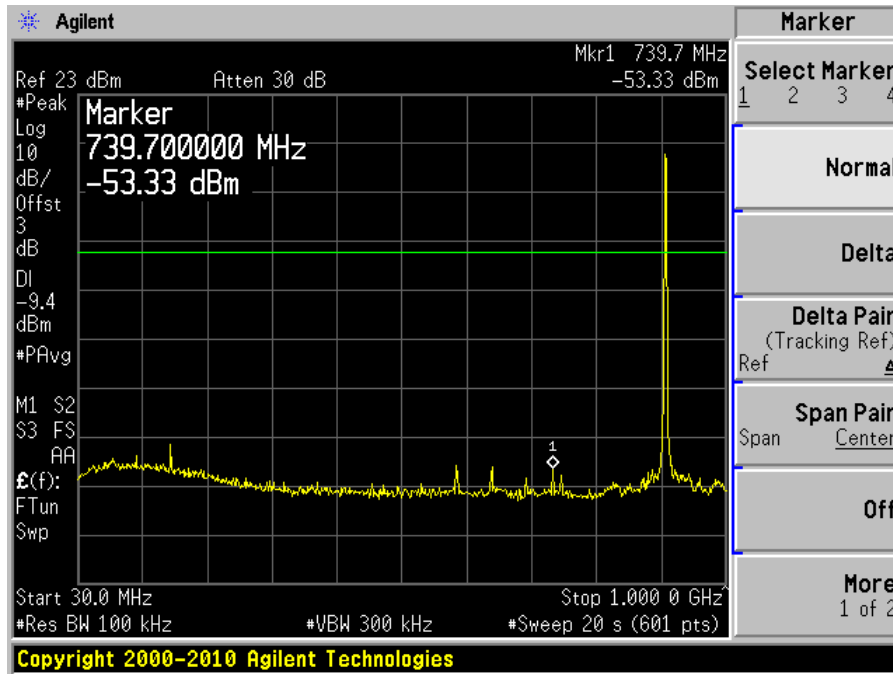
Plot 1: 30 MHz~1GHz
