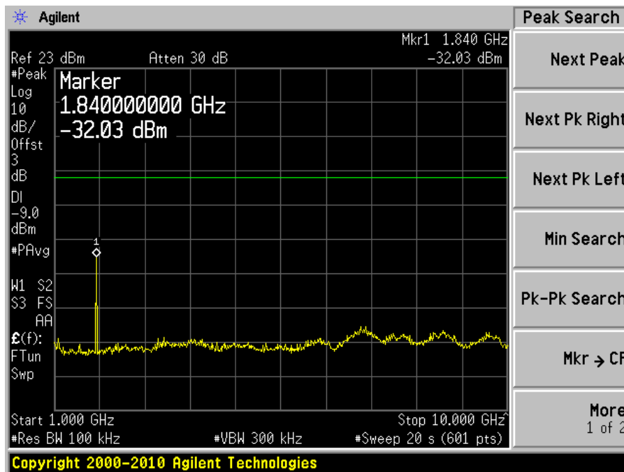
Plot 2: 1 ~ 10 GHz
