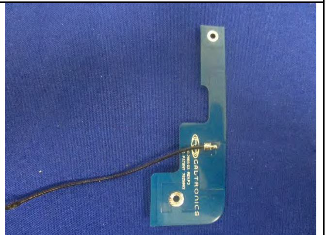
Internal antenna 1
