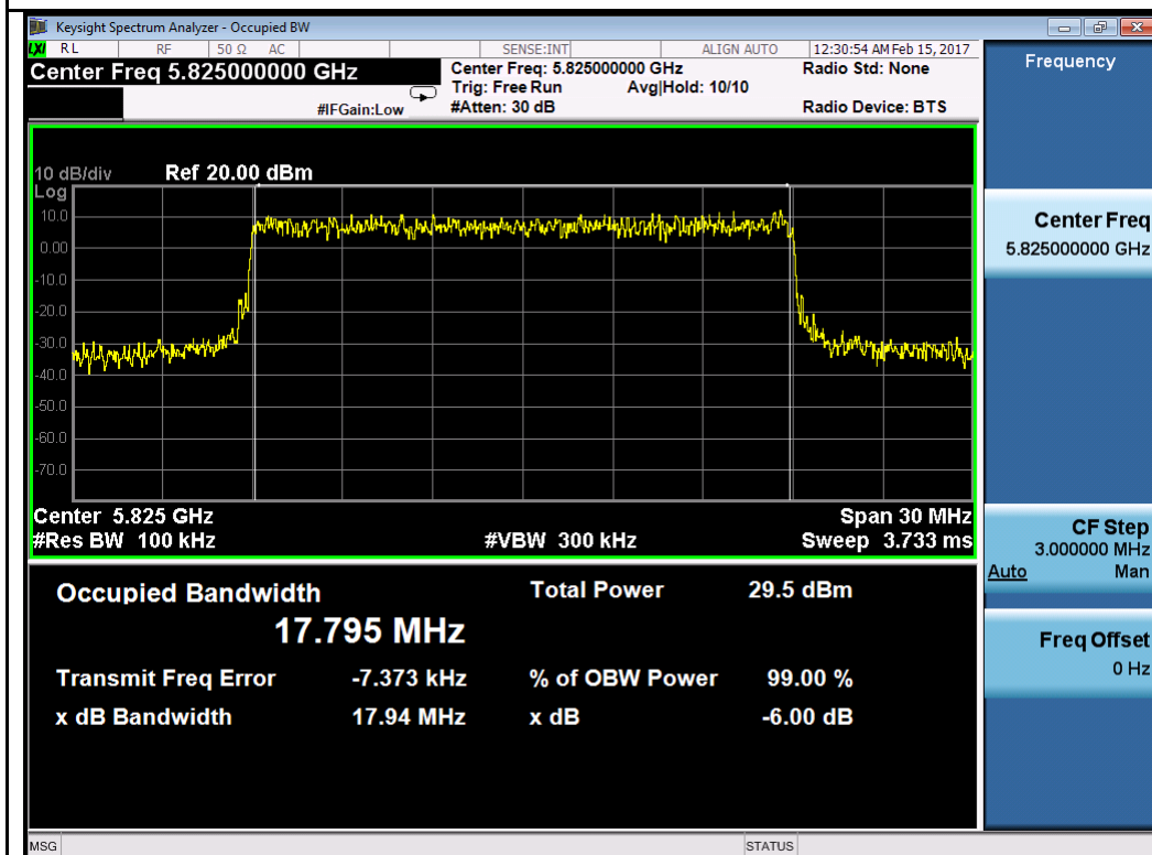
64QAM-5825MHz
