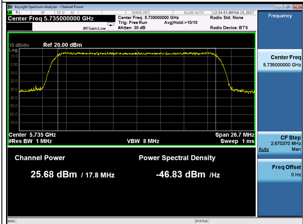
64QAM-5735MHz
