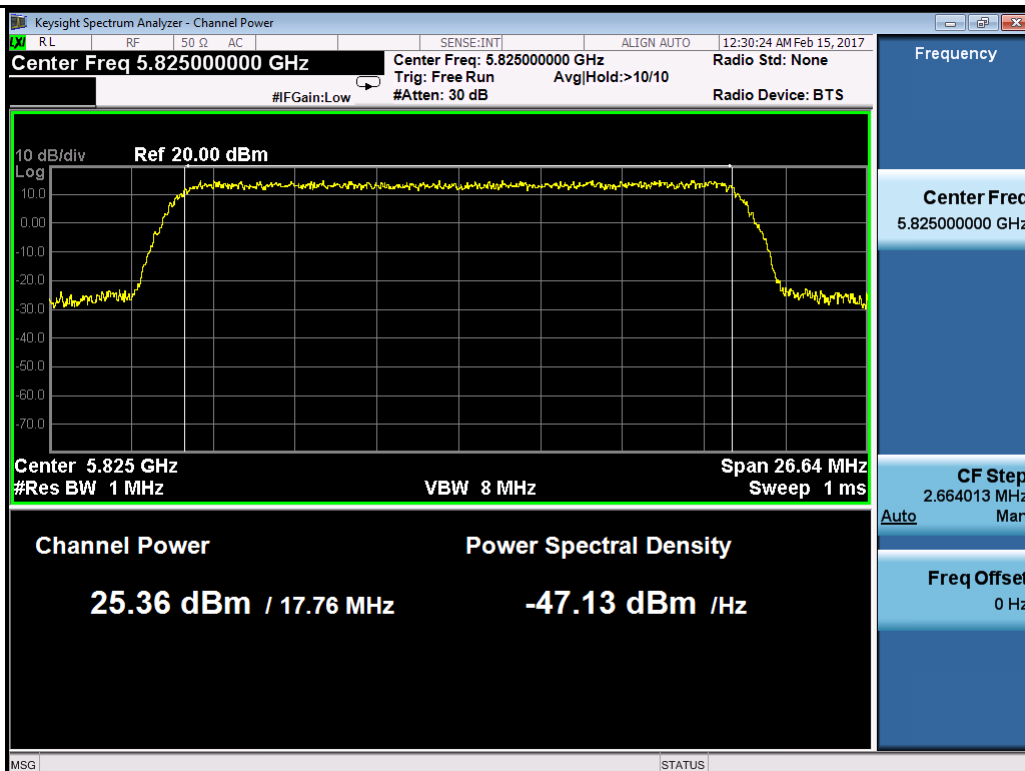
64QAM-5825MHz
