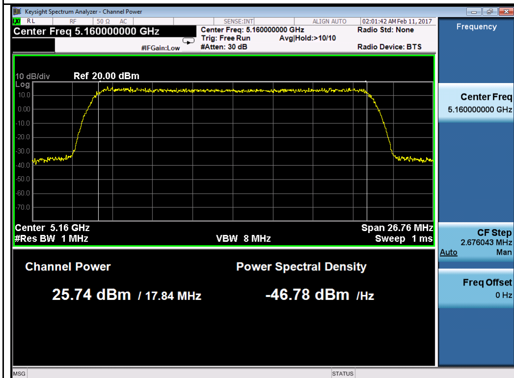
64QAM-5160MHz
