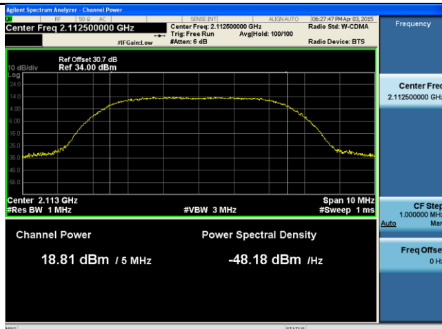
PWR-Band4-64QAM-5M BW-Low CH-Port1
