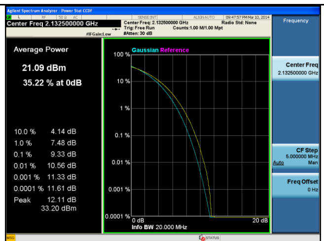
PK-AV-Ratio-Band4-64QAM-20M BW-Mid
