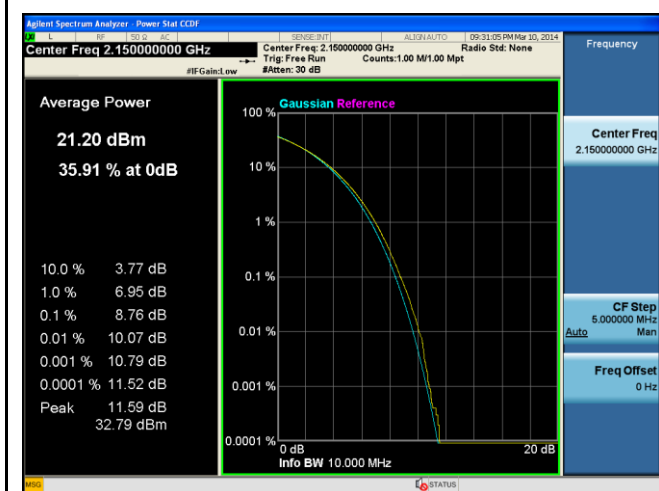
PK-AV-Ratio-Band4-64QAM-10M BW-High
