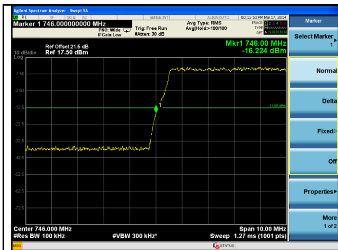
BandEdge-LTE-Band13-10MHz-QPSK-Low
