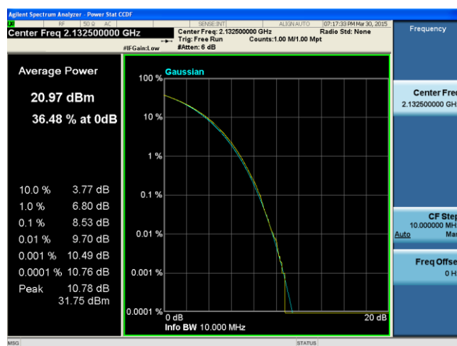
PK-AV-Ratio-Band4-QPSK-15M BW-Mid
