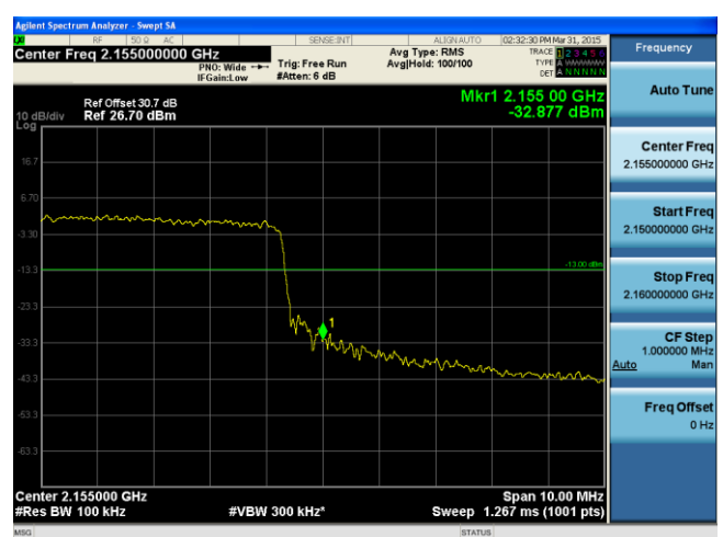
BandEdge-LTE-Band4-15MHz-64QAM-High
