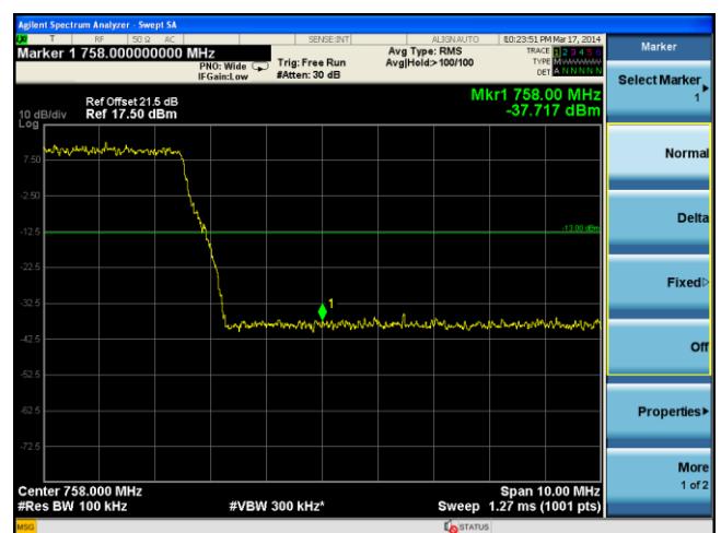
BandEdge-LTE-Band13-10MHz-64QAM-High
