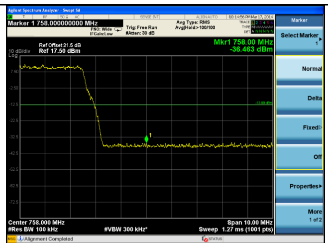
BandEdge-LTE-Band13-10MHz-QPSK-High
