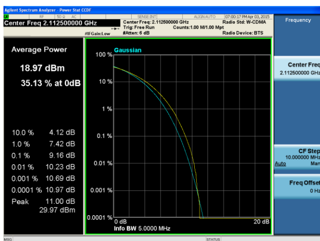
PK-AV-Ratio-Band4-QPSK-5M BW-Low
