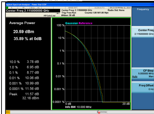
PK-AV-Ratio-Band4-64QAM-10M BW-Low
