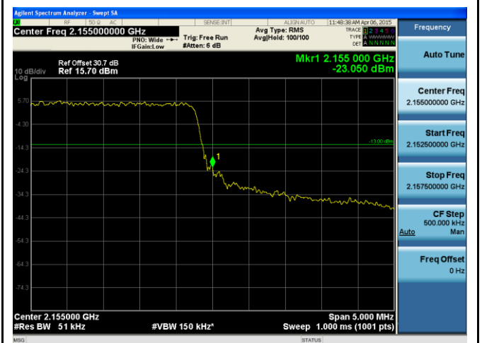
BandEdge-LTE-Band4-5MHz-64QAM-High
