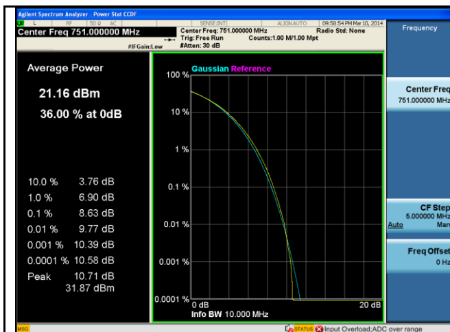
PK-AV-Ratio-Band13-QPSK-10M BW-Mid
