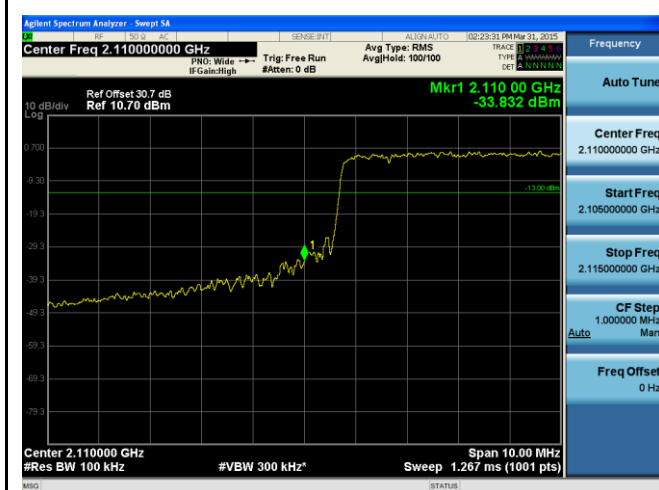
BandEdge-LTE-Band4-15MHz-64QAM-Low
