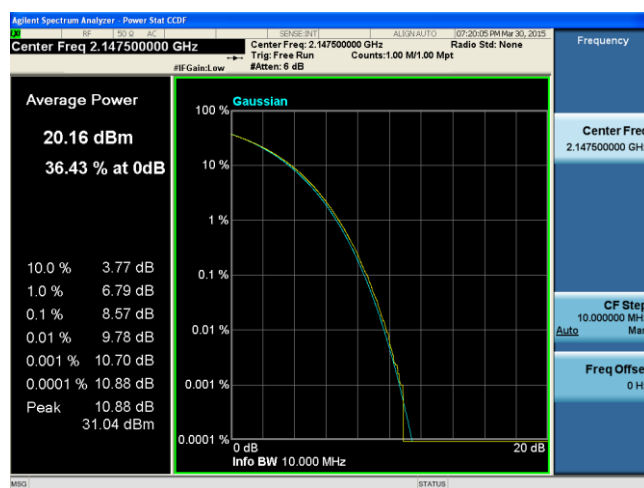
PK-AV-Ratio-Band4-QPSK-15M BW-High
