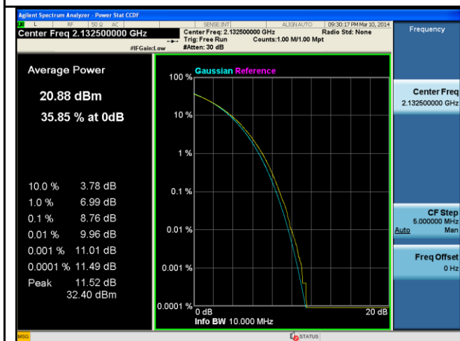
PK-AV-Ratio-Band4-64QAM-10M BW-Mid
