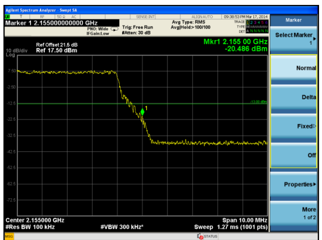
BandEdge-LTE-Band4-20MHz-64QAM-High
