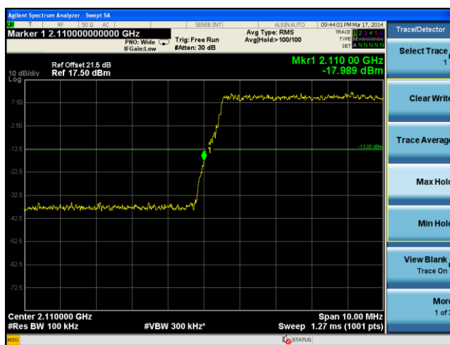
BandEdge-LTE-Band4-10MHz-64QAM-Low
