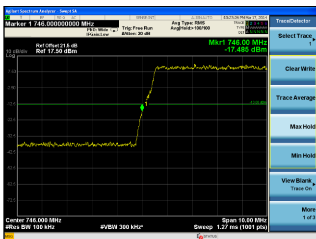
BandEdge-LTE-Band13-10MHz-64QAM-Low
