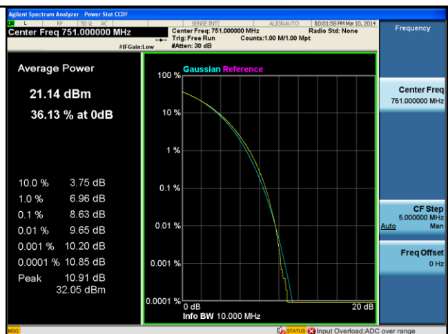
PK-AV-Ratio-Band13-16QAM-10M BW-Mid
