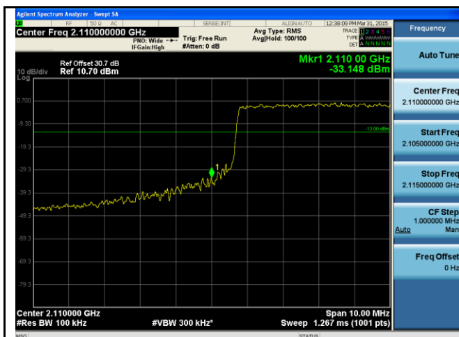
BandEdge-LTE-Band4-15MHz-QPSK-Low
