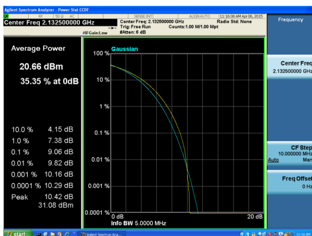
PK-AV-Ratio-Band4-QPSK-5M BW-Mid
