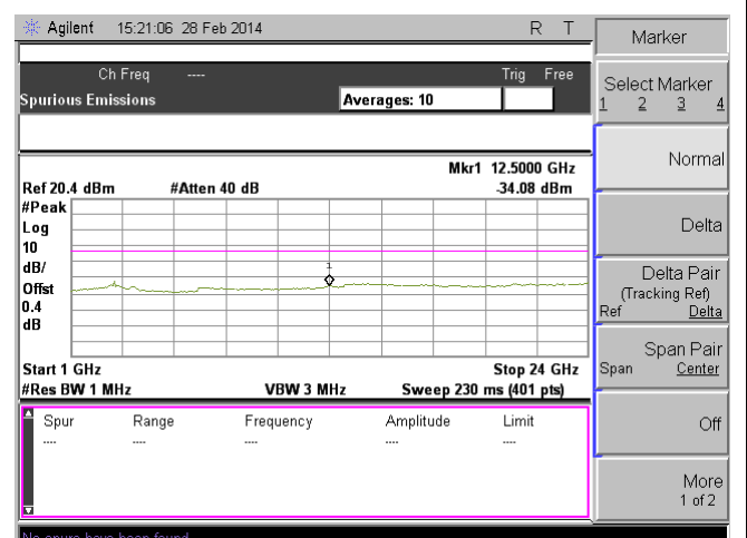
TX CSE-Band13-64QAM-10M BW-Mid CH-above 1G
