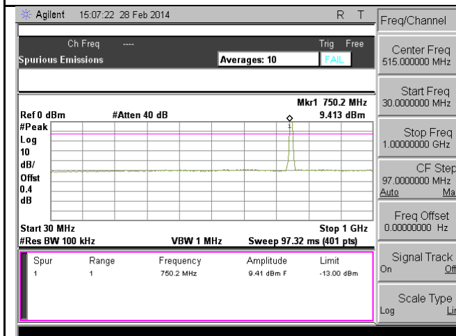
TX CSE-Band13-16QAM-10M BW-Mid CH-below 1G
