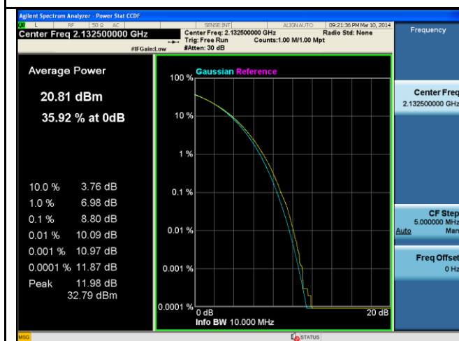
PK-AV-Ratio-Band4-16QAM-10M BW-Mid
