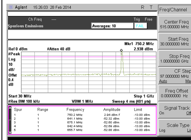
TX CSE-Band13-64QAM-10M BW-Mid CH-below 1G
