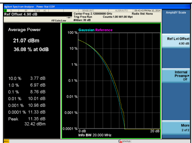
PK-AV-Ratio-Band4-16QAM-20M BW-Low
