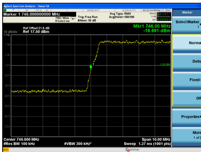
BandEdge-LTE-Band13-10MHz-16QAM-Low
