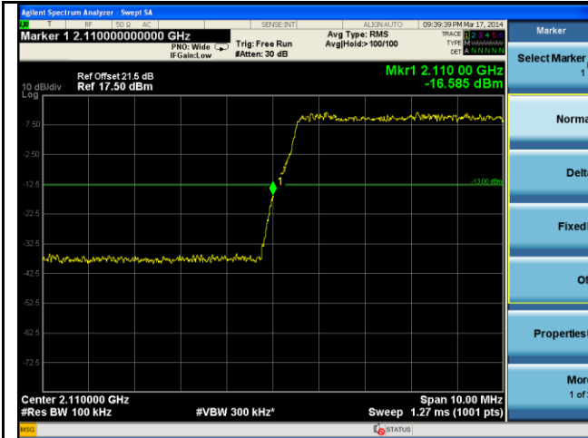
BandEdge-LTE-Band4-10MHz-QPSK-Low
