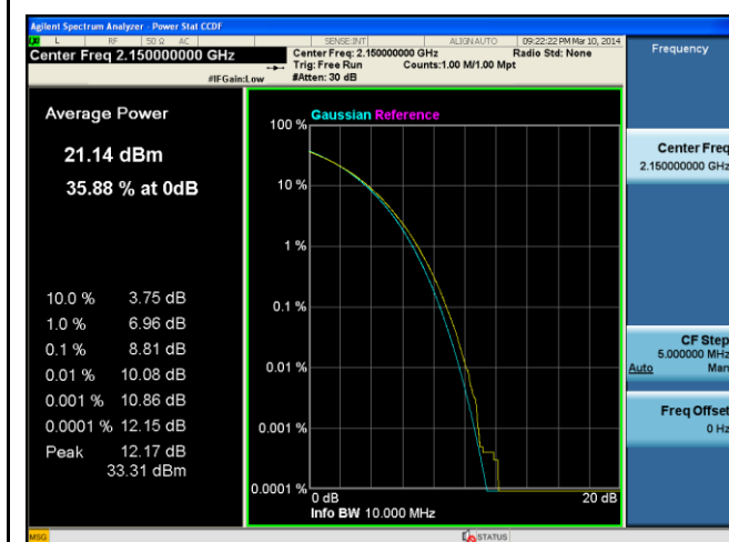
PK-AV-Ratio-Band4-16QAM-10M BW-High
