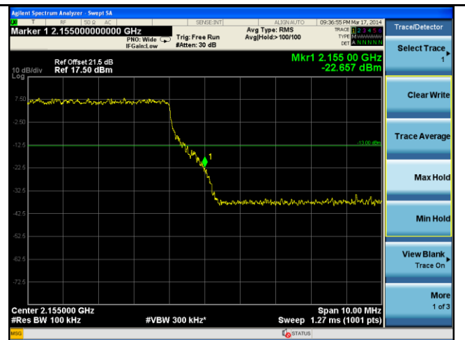
BandEdge-LTE-Band4-20MHz-16QAM-High
