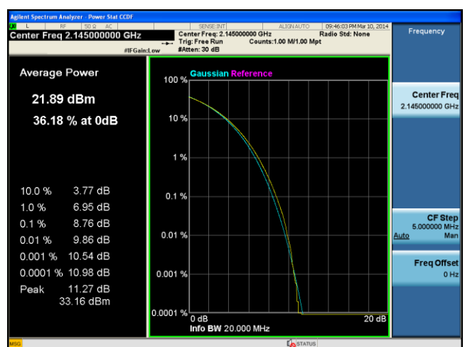
PK-AV-Ratio-Band4-16QAM-20M BW-High
