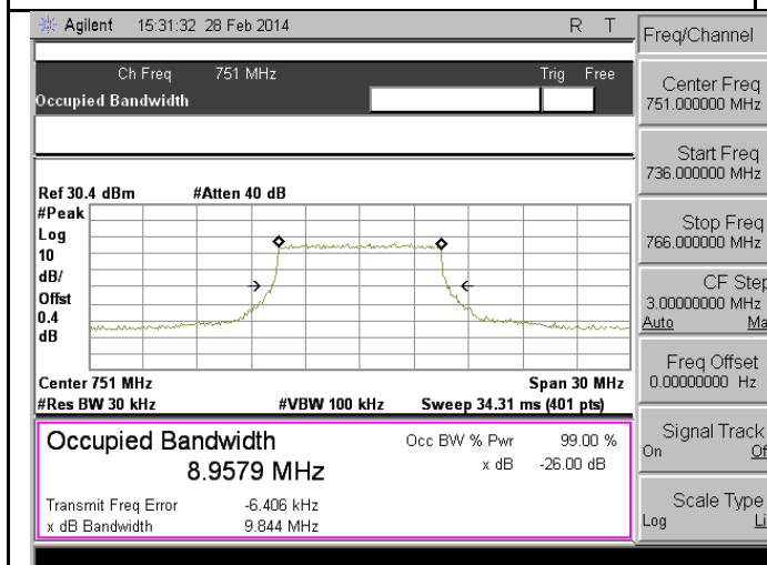
OBW-Band13-Mid-64QAM
