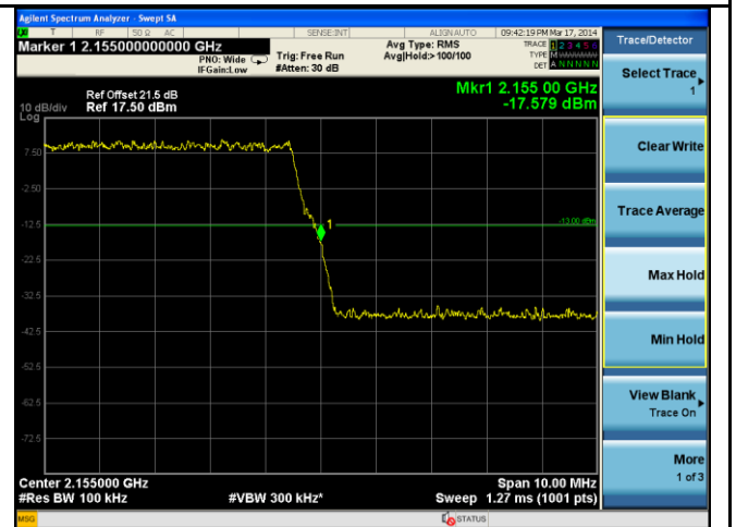
BandEdge-LTE-Band4-10MHz-16QAM-High
