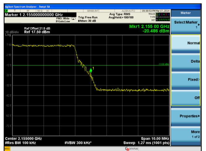
BandEdge-LTE-Band4-20MHz-64QAM-High
