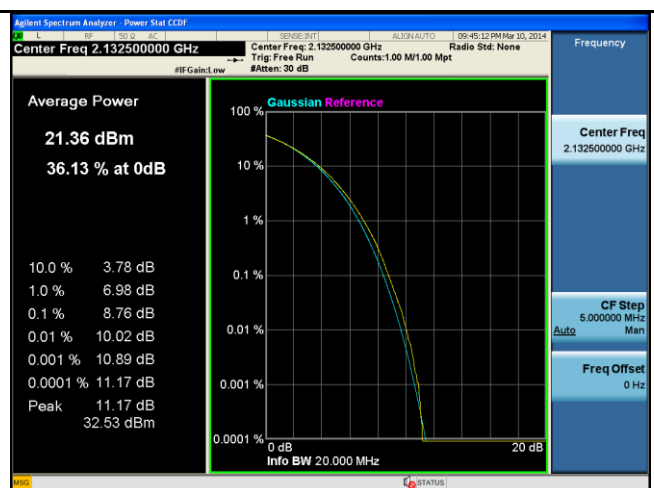
PK-AV-Ratio-Band4-16QAM-20M BW-Mid
