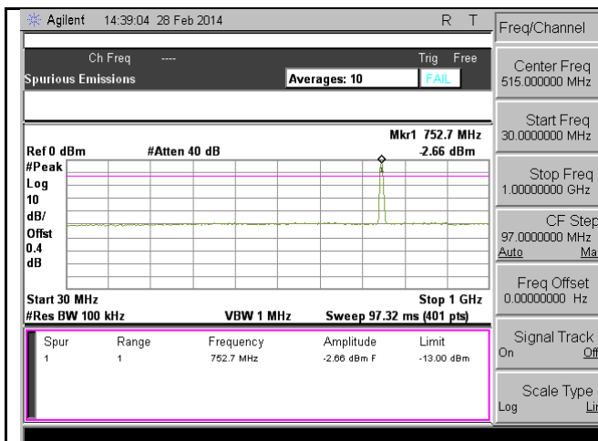
TX CSE-Band13-QPSK-10M BW-Mid CH-below 1G
