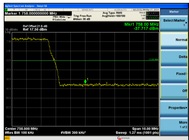
BandEdge-LTE-Band13-10MHz-64QAM-High
