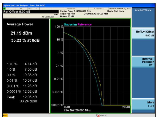
PK-AV-Ratio-Band4-64QAM-20M BW-High
