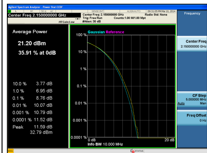
PK-AV-Ratio-Band4-64QAM-10M BW-High
