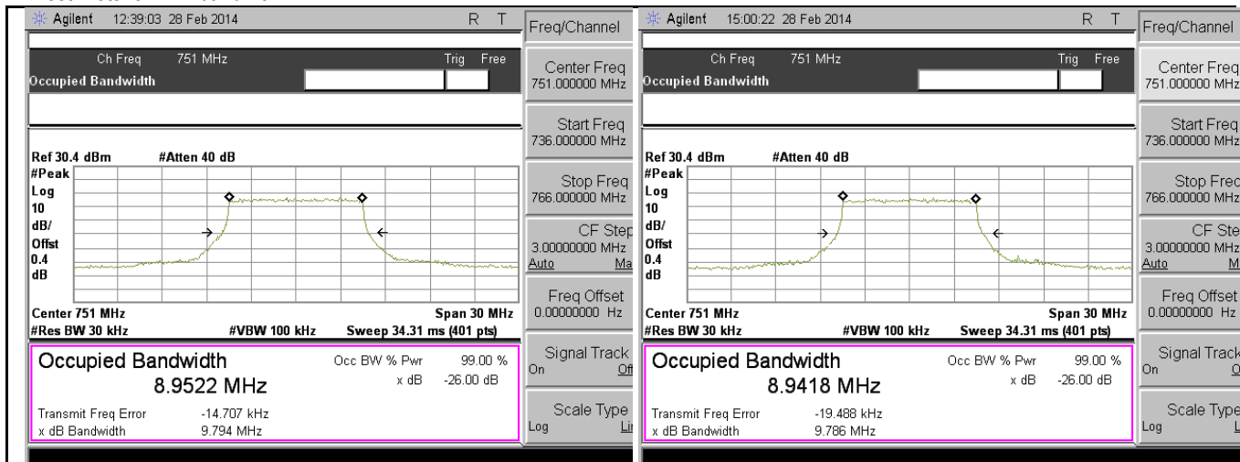
OBW-Band13-Mid-QPSK
