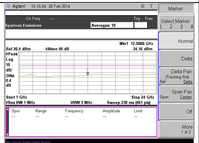
TX CSE-Band13-16QAM-10M BW-Mid CH-above 1G
