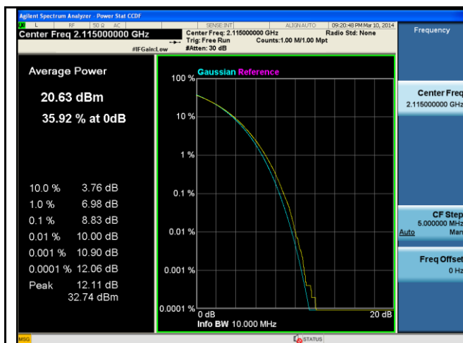
PK-AV-Ratio-Band4-16QAM-10M BW-Low
