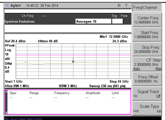
TX CSE-Band13-QPSK-10M BW-Mid CH-above 1G
