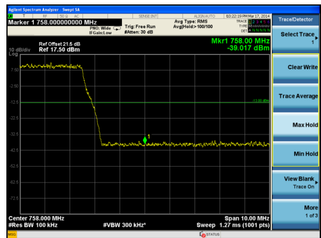
BandEdge-LTE-Band13-10MHz-16QAM-High
