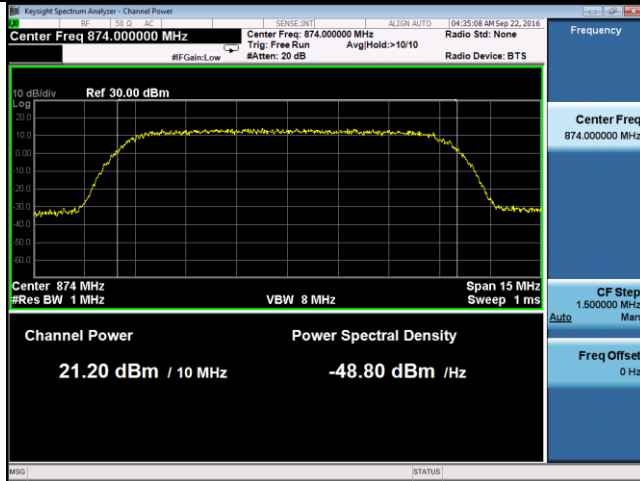
PWR- Band5-64QAM-10M BW-Low CH-Port1
