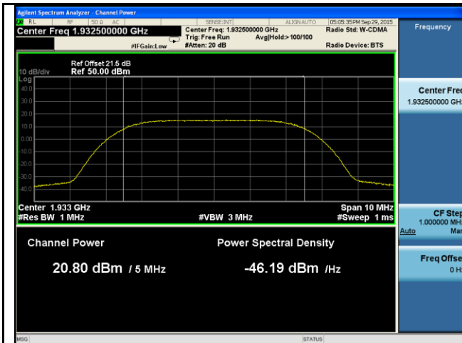
PWR- Band2-64QAM-5M BW-Low CH-Port1
