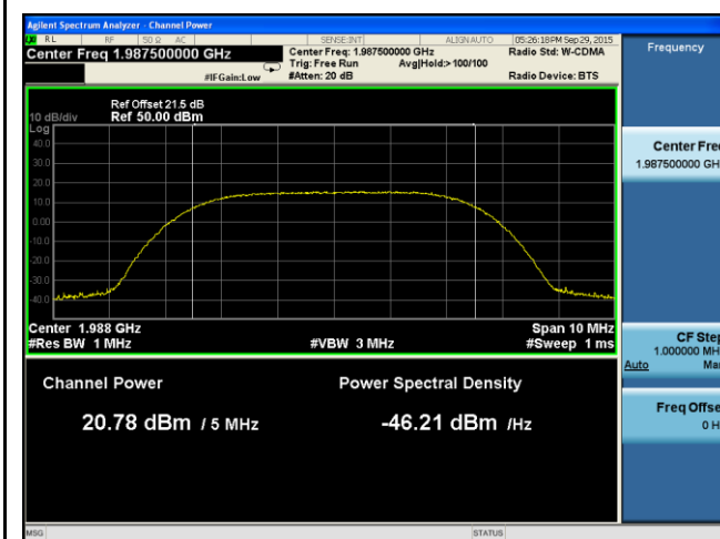
PWR- Band2-64QAM-5M BW-High CH-Port1
