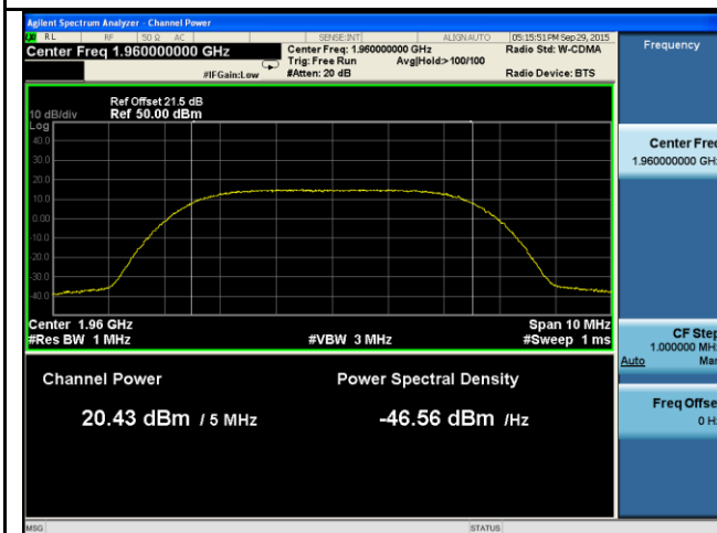
PWR- Band2-64QAM-5M BW-Mid CH-Port1
