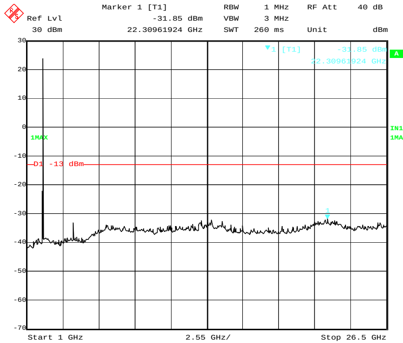
Spurious Emission at Antenna Port, High Channel, 1GHz to 26GHz
