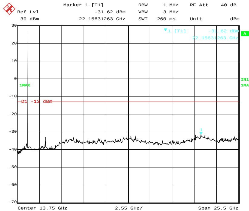
Spurious Emission at Antenna Port, Mid Channel, 1GHz to 26GHz
