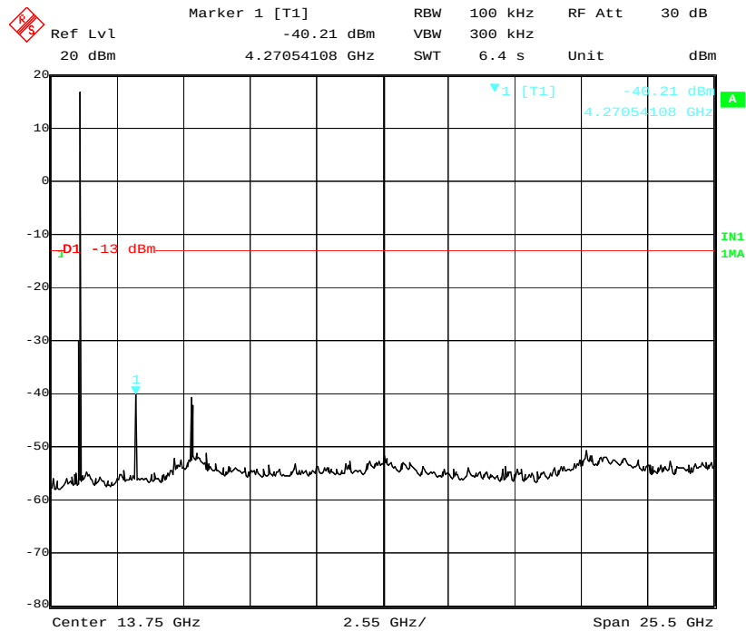
Spurious Emission at Antenna Port, Low Channel, 1GHz to 26GHz
