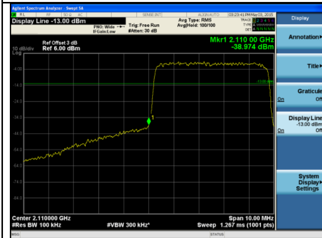
BandEdge-LTE-Band4-5MHz-16QAM-Low
