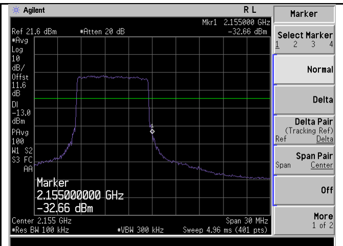
BandEdge-LTE-Band4-10MHz-QPSK-High
