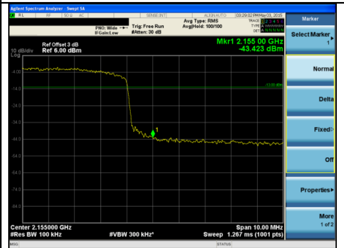
BandEdge-LTE-Band4-20MHz-16QAM-High
