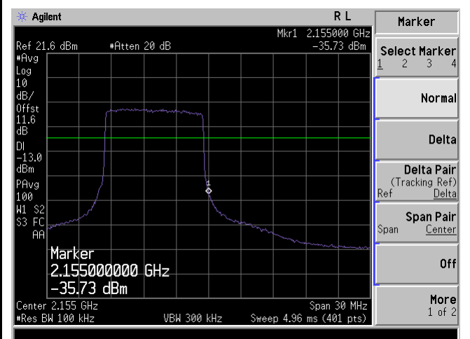
BandEdge-LTE-Band4-10MHz-64QAM-High
