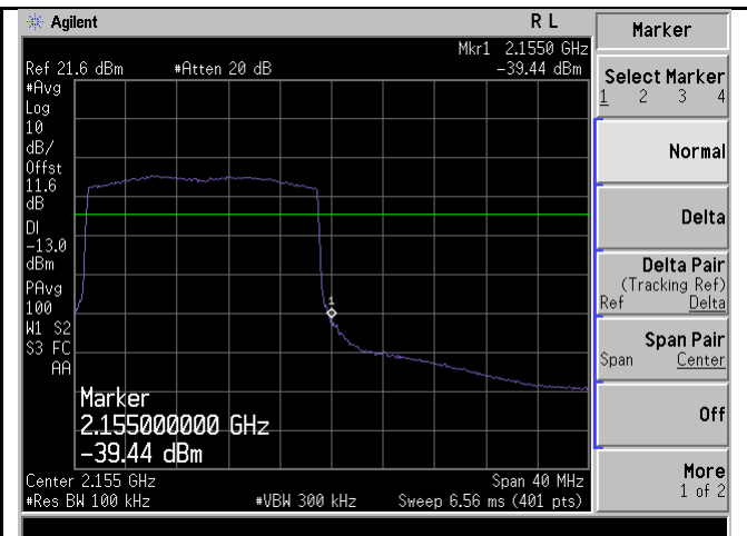
BandEdge-LTE-Band4-20MHz-QPSK-High
