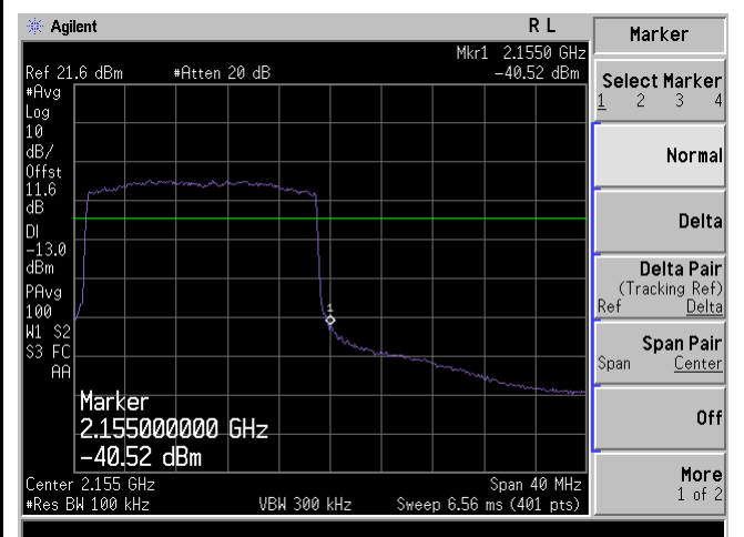
BandEdge-LTE-Band4-20MHz-64QAM-High
