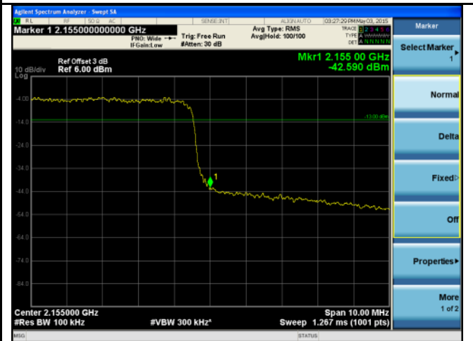
BandEdge-LTE-Band4-10MHz-16QAM-High
