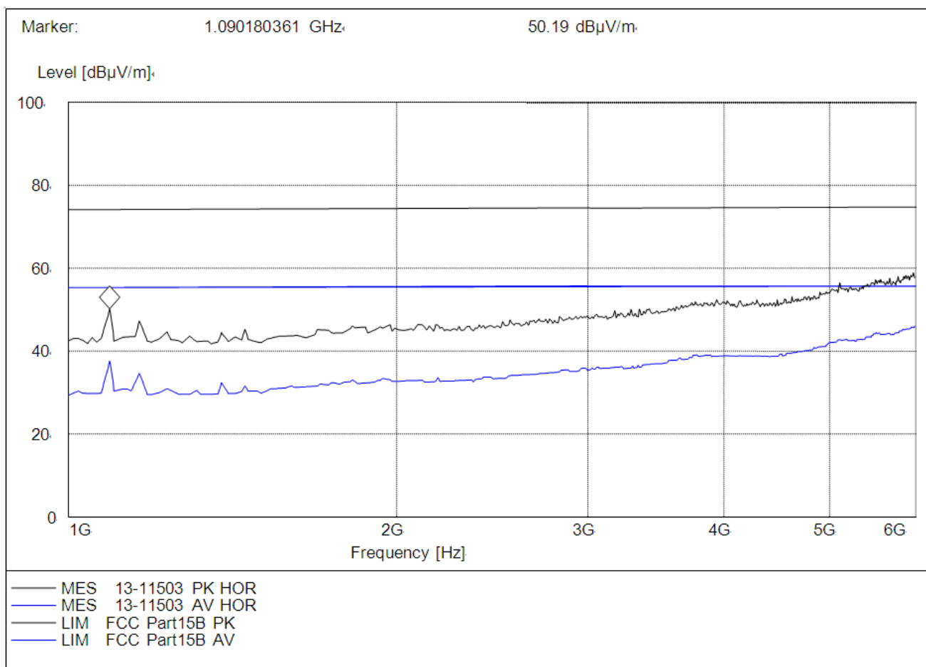
(Plot C: Test Antenna Horizontal 1G – 6G)
