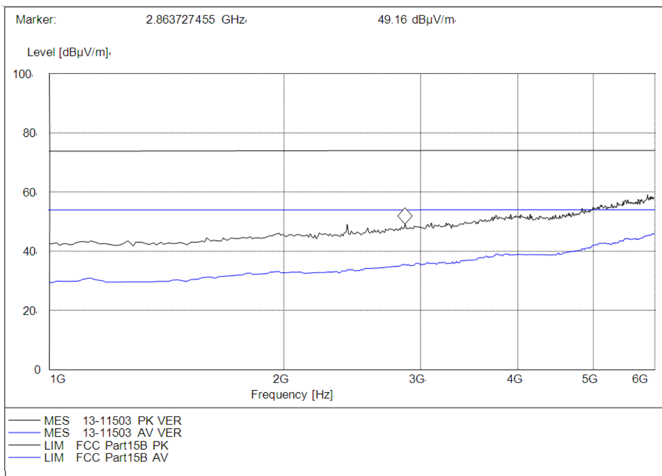
(Plot D: Test Antenna Vertical 1G – 6G)
