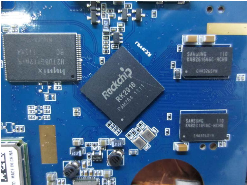
INTERNAL PHOTO OF 7 inch SAMPLE-8
