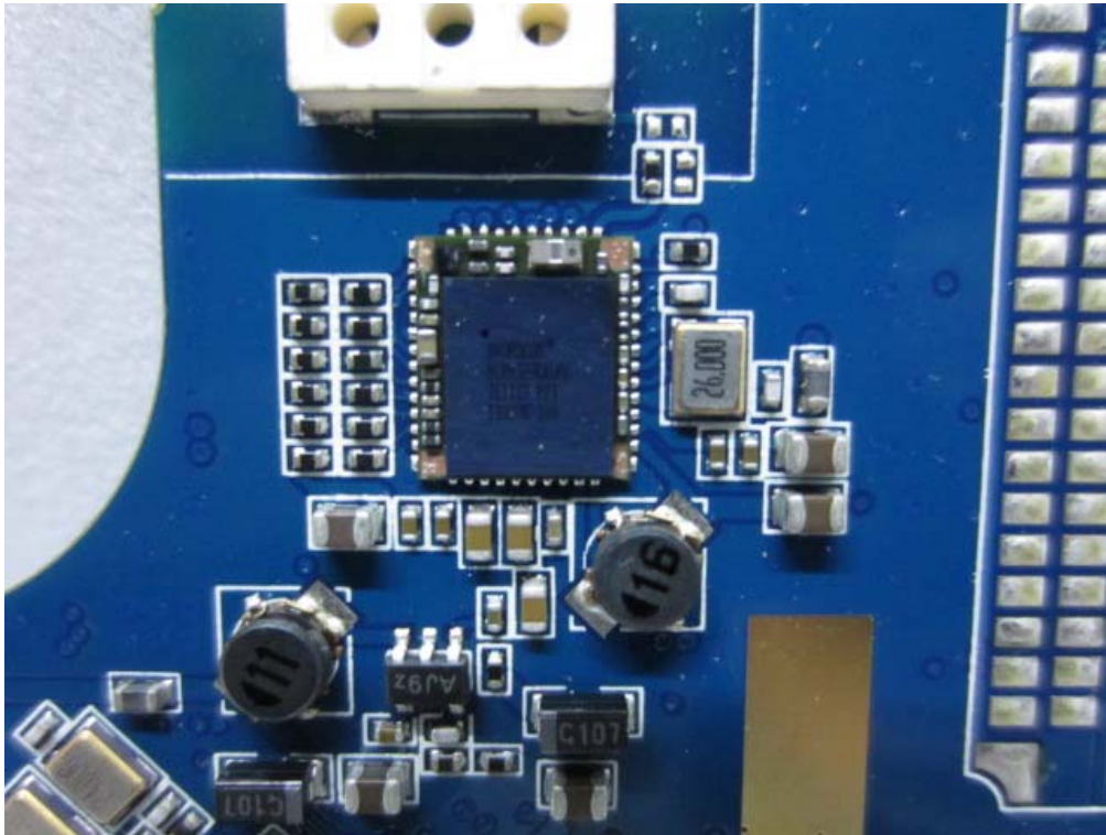
INTERNAL PHOTO OF 7 inch SAMPLE – 11
