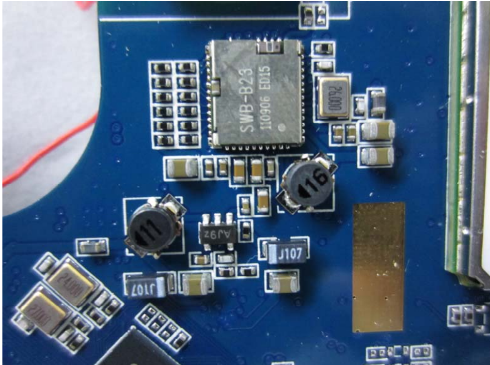
INTERNAL PHOTO OF 7 inch SAMPLE – 10
