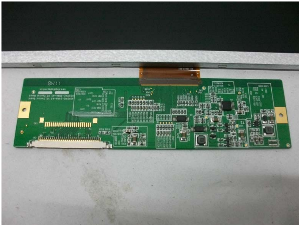
INTERNAL PHOTO OF 7 inch SAMPLE -6
