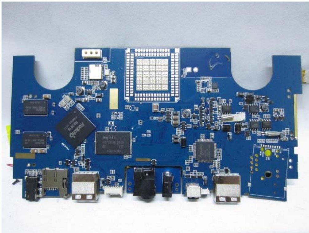
INTERNAL PHOTO OF 7 inch SAMPLE -4
