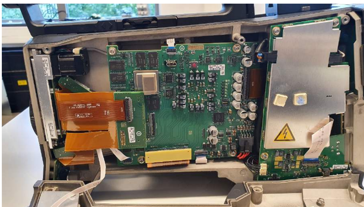
1.2 Side 2 PCB view
