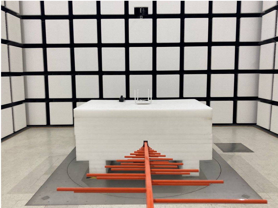
Radiated Emission Below 1GHz View AX1500M
