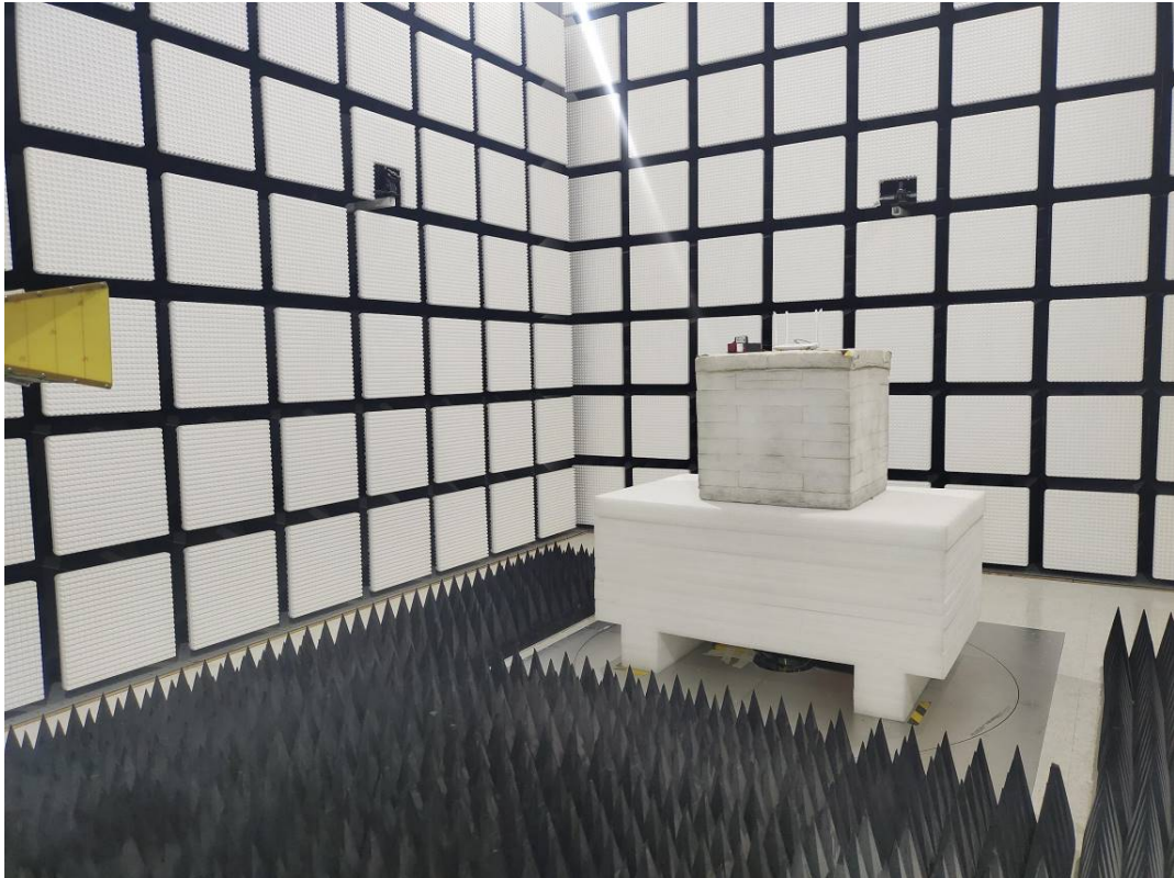
Radiated Emission Above 1GHz View AX1500MS
